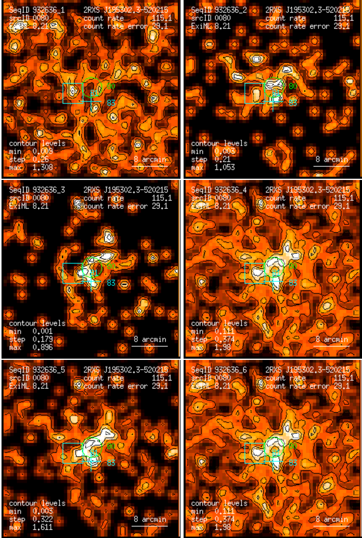
Figure 80: RASS 932636: detection 0080: band rate images, Gaussian filter: (1) PSPC channels 11 – 41, (2) 52 – 90, (3) 91 – 201, (4) 11 – 235, (5) 52 – 201, (6) 11 – 201. Broad band rates in counts/ks. Band rate contour levels in counts/ks/arcmin 2 .
