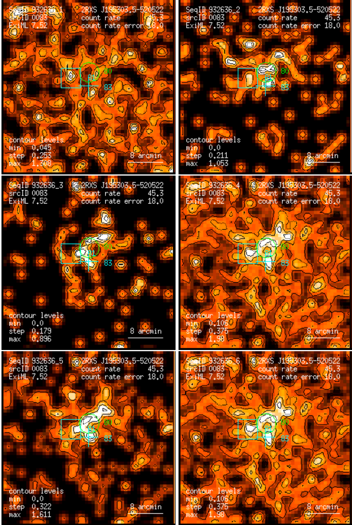
Figure 83: RASS 932636: detection 0083: band rate images, Gaussian filter: (1) PSPC channels 11 – 41, (2) 52 – 90, (3) 91 – 201, (4) 11 – 235, (5) 52 – 201, (6) 11 – 201. Broad band rates in counts/ks. Band rate contour levels in counts/ks/arcmin 2 .
