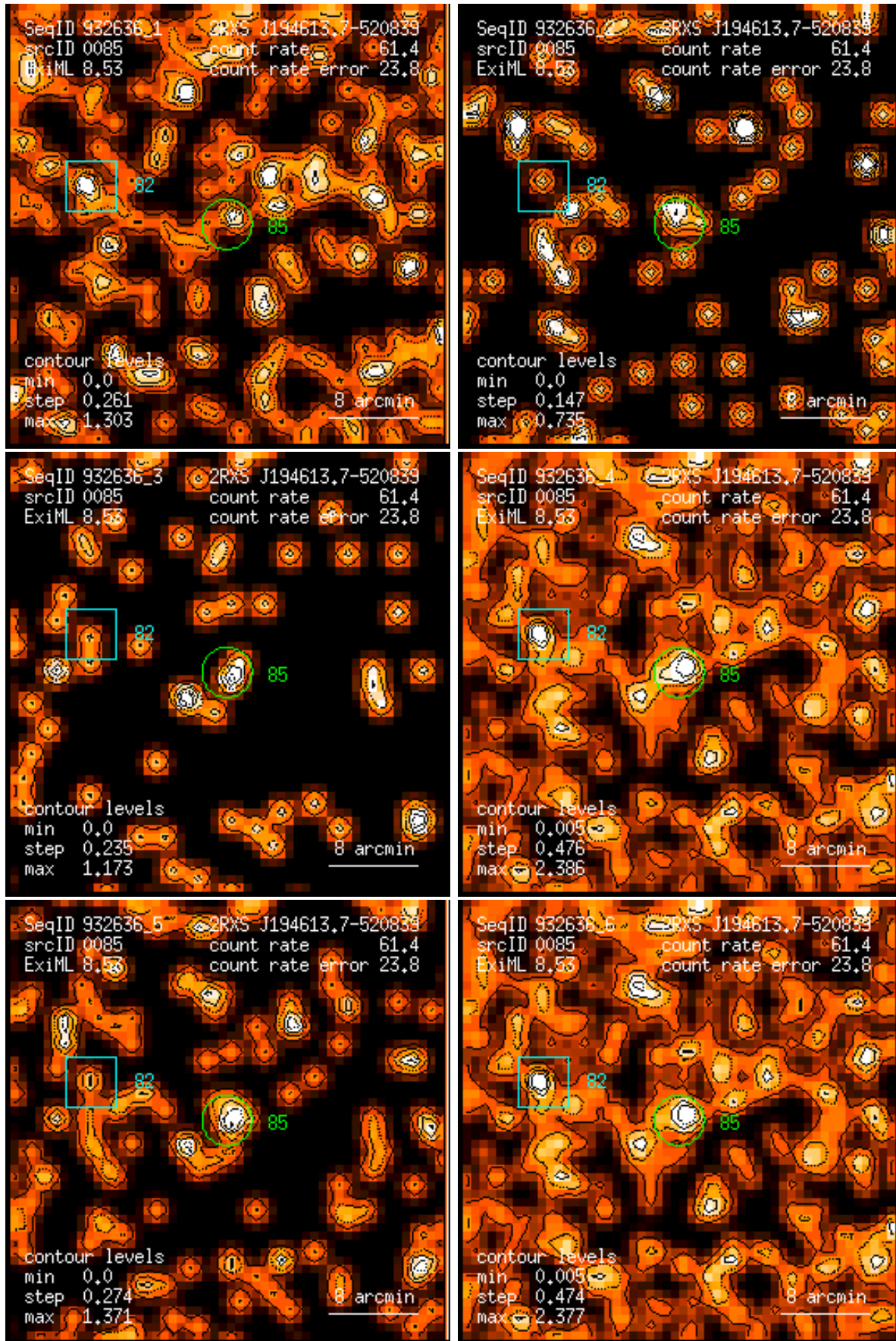
Figure 85: RASS 932636: detection 0085: band rate images, Gaussian filter: (1) PSPC channels 11 – 41, (2) 52 – 90, (3) 91 – 201, (4) 11 – 235, (5) 52 – 201, (6) 11 – 201. Broad band rates in counts/ks. Band rate contour levels in counts/ks/arcmin 2 .
