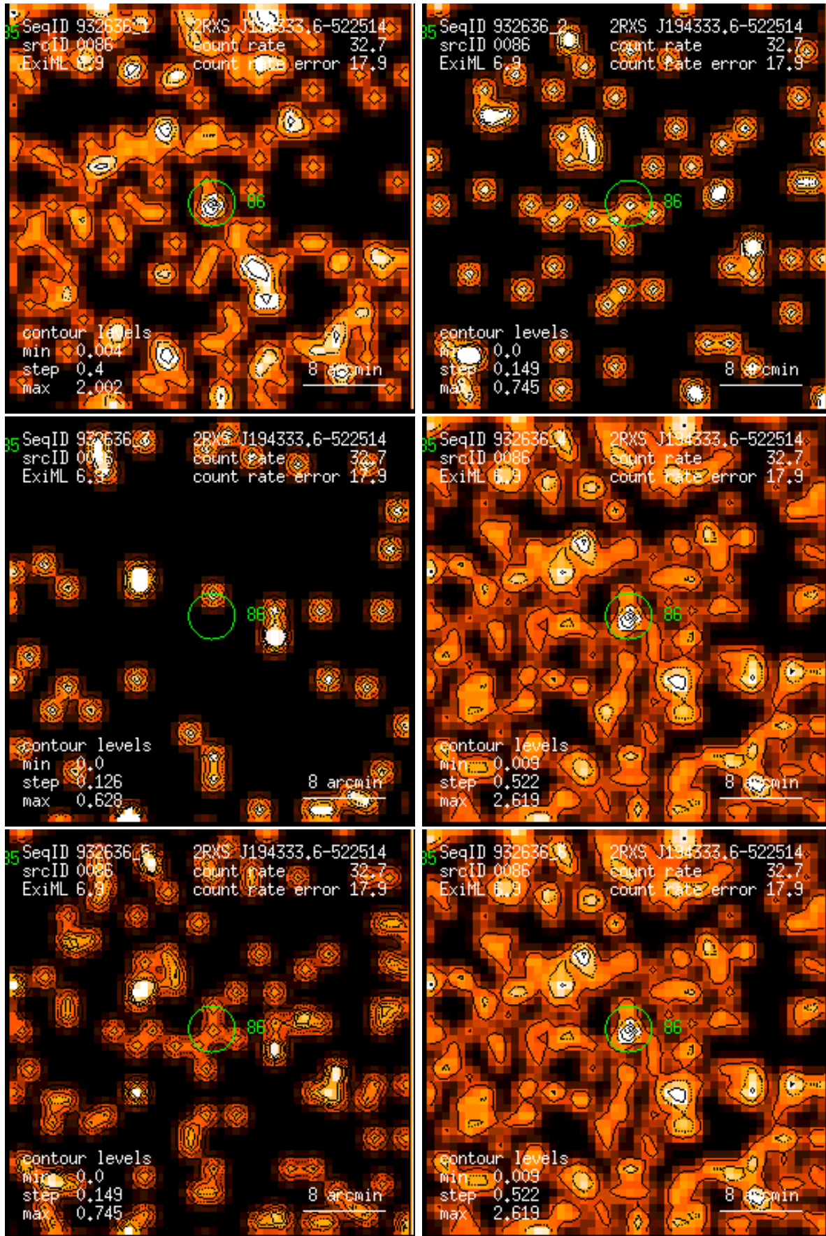
Figure 86: RASS 932636: detection 0086: band rate images, Gaussian filter: (1) PSPC channels 11 – 41, (2) 52 – 90, (3) 91 – 201, (4) 11 – 235, (5) 52 – 201, (6) 11 – 201. Broad band rates in counts/ks. Band rate contour levels in counts/ks/arcmin 2 .
