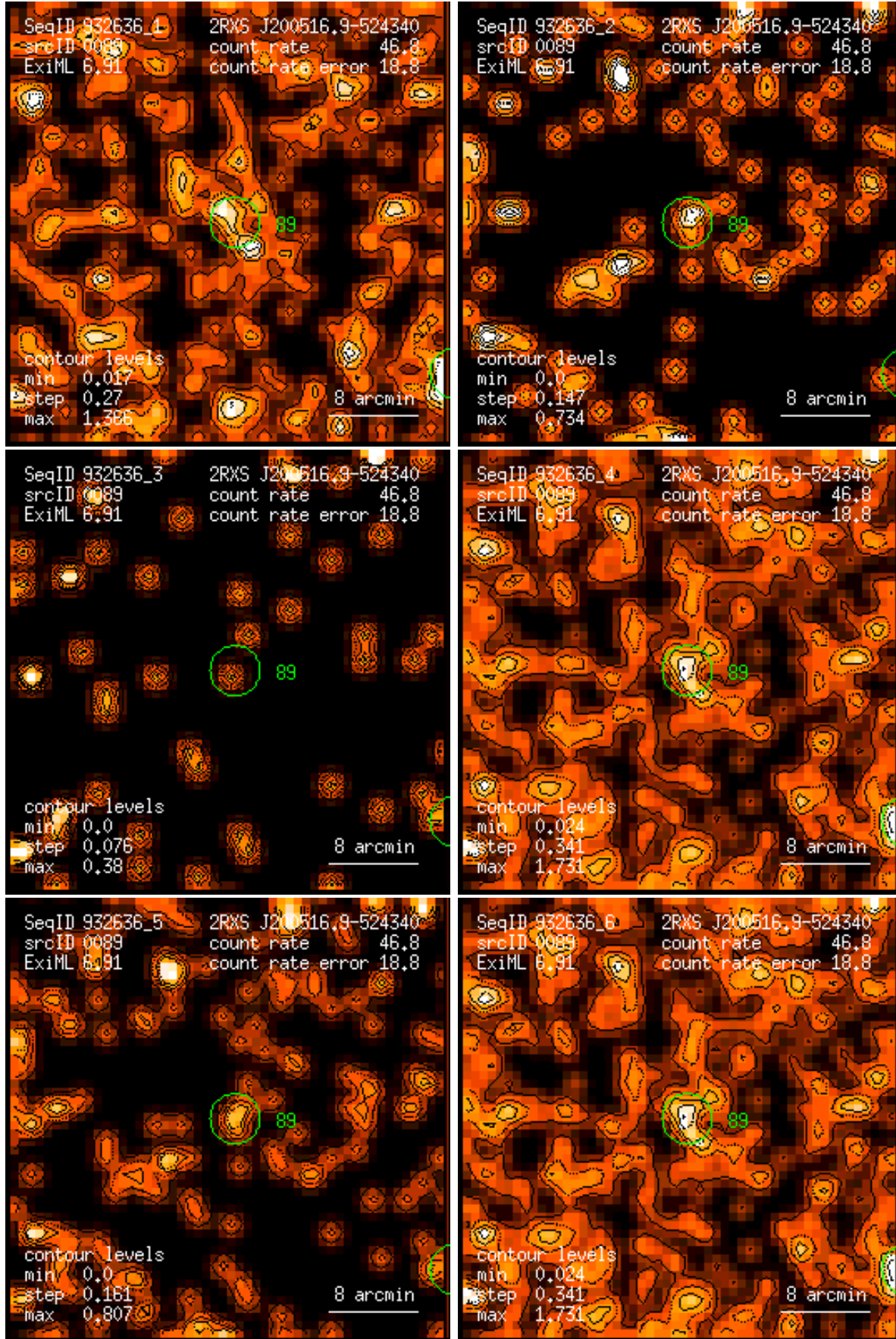
Figure 89: RASS 932636: detection 0089: band rate images, Gaussian filter: (1) PSPC channels 11 – 41, (2) 52 – 90, (3) 91 – 201, (4) 11 – 235, (5) 52 – 201, (6) 11 – 201. Broad band rates in counts/ks. Band rate contour levels in counts/ks/arcmin 2 .
