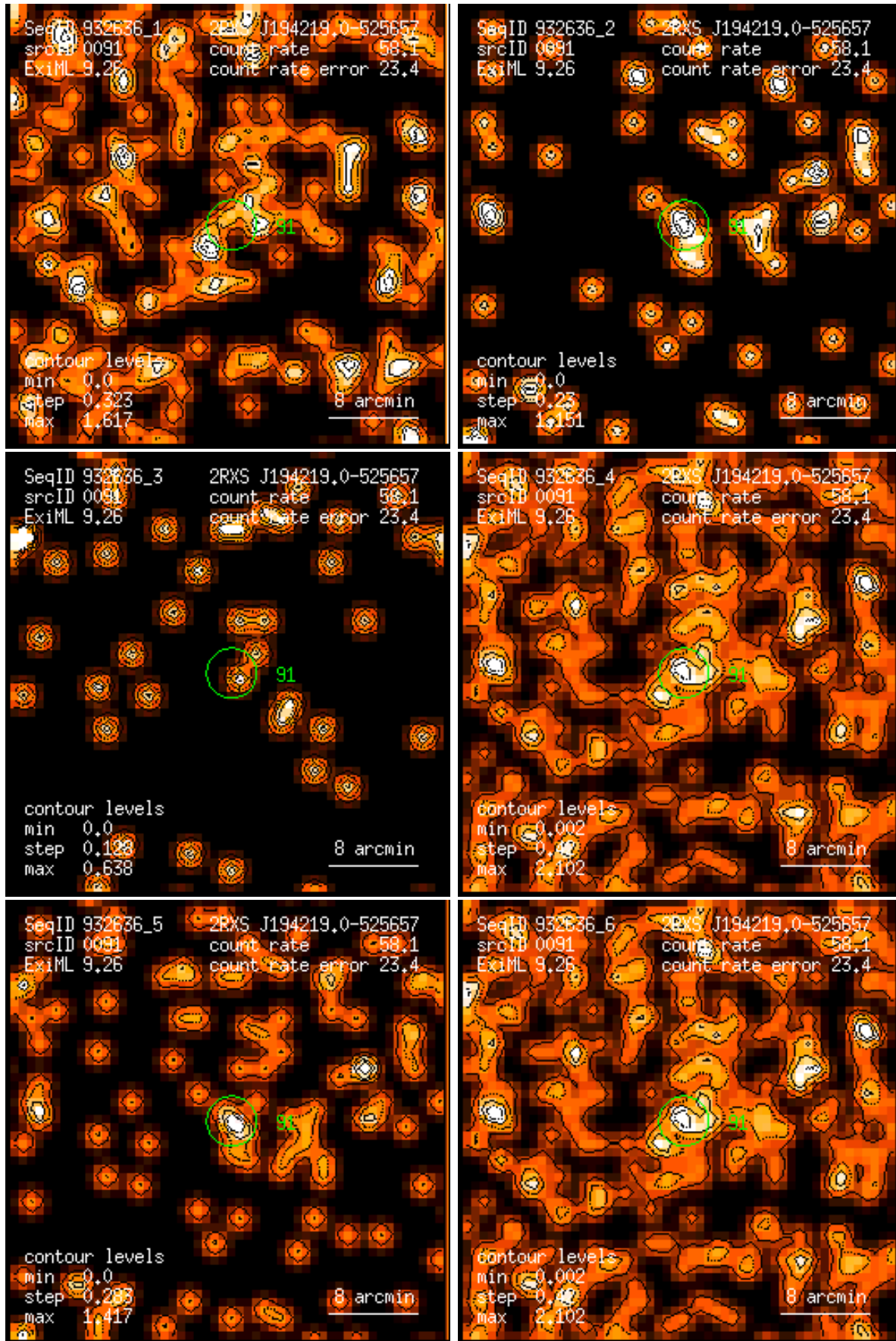
Figure 91: RASS 932636: detection 0091: band rate images, Gaussian filter: (1) PSPC channels 11 – 41, (2) 52 – 90, (3) 91 – 201, (4) 11 – 235, (5) 52 – 201, (6) 11 – 201. Broad band rates in counts/ks. Band rate contour levels in counts/ks/arcmin 2 .
