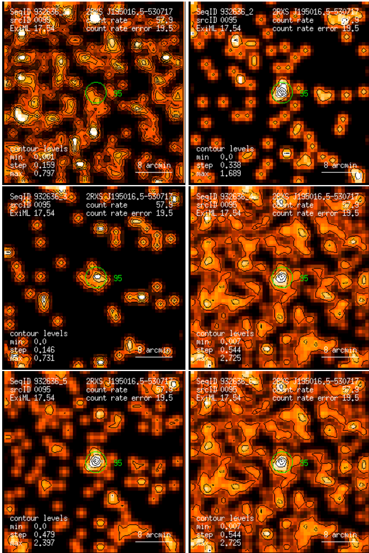
Figure 95: RASS 932636: detection 0095: band rate images, Gaussian filter: (1) PSPC channels 11 – 41, (2) 52 – 90, (3) 91 – 201, (4) 11 – 235, (5) 52 – 201, (6) 11 – 201. Broad band rates in counts/ks. Band rate contour levels in counts/ks/arcmin 2 .
