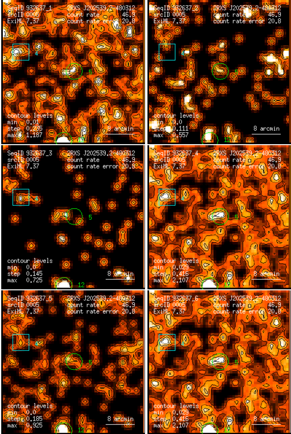
Figure 5: RASS 932637: detection 0005: band rate images, Gaussian filter: (1) PSPC channels 11 – 41, (2) 52 – 90, (3) 91 – 201, (4) 11 – 235, (5) 52 – 201, (6) 11 – 201. Broad band rates in counts/ks. Band rate contour levels in counts/ks/arcmin 2 .
