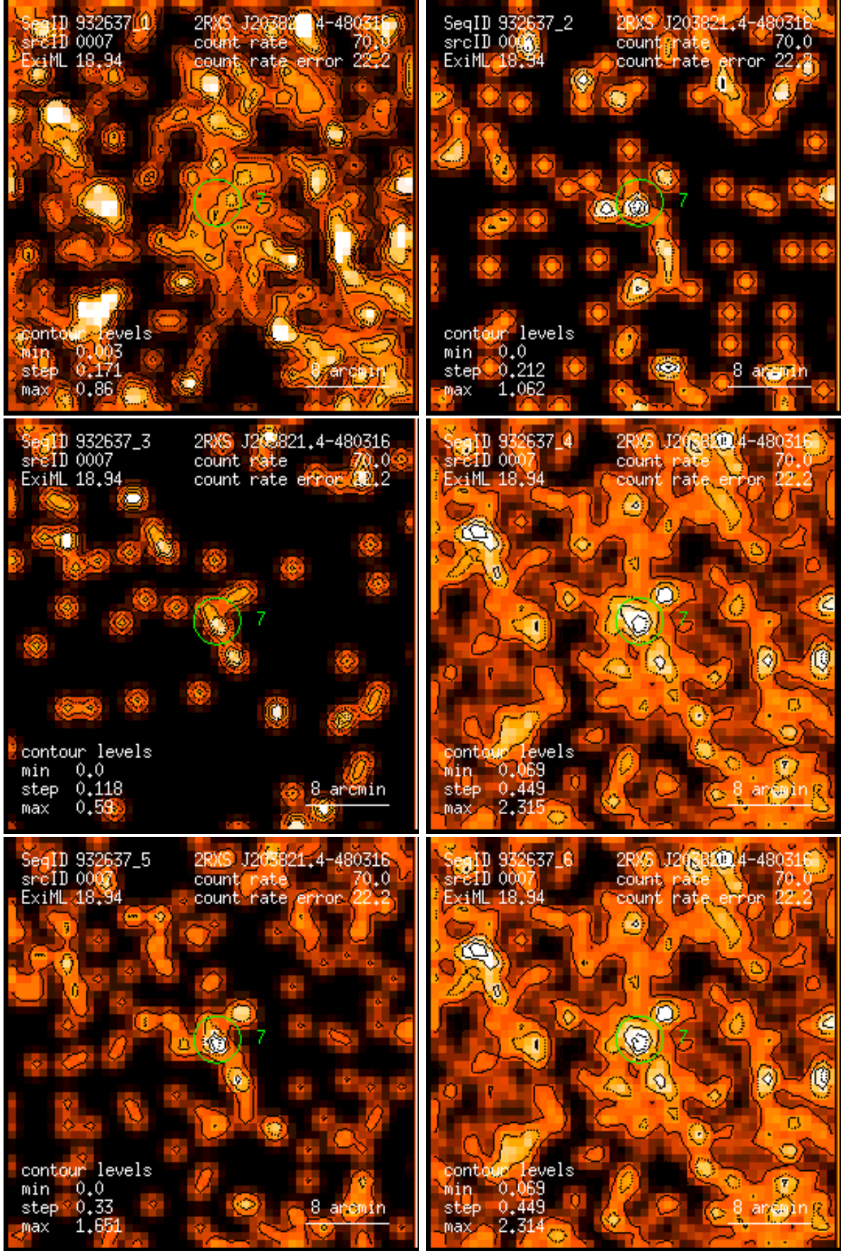
Figure 7: RASS 932637: detection 0007: band rate images, Gaussian filter: (1) PSPC channels 11 – 41, (2) 52 – 90, (3) 91 – 201, (4) 11 – 235, (5) 52 – 201, (6) 11 – 201. Broad band rates in counts/ks. Band rate contour levels in counts/ks/arcmin 2 .
