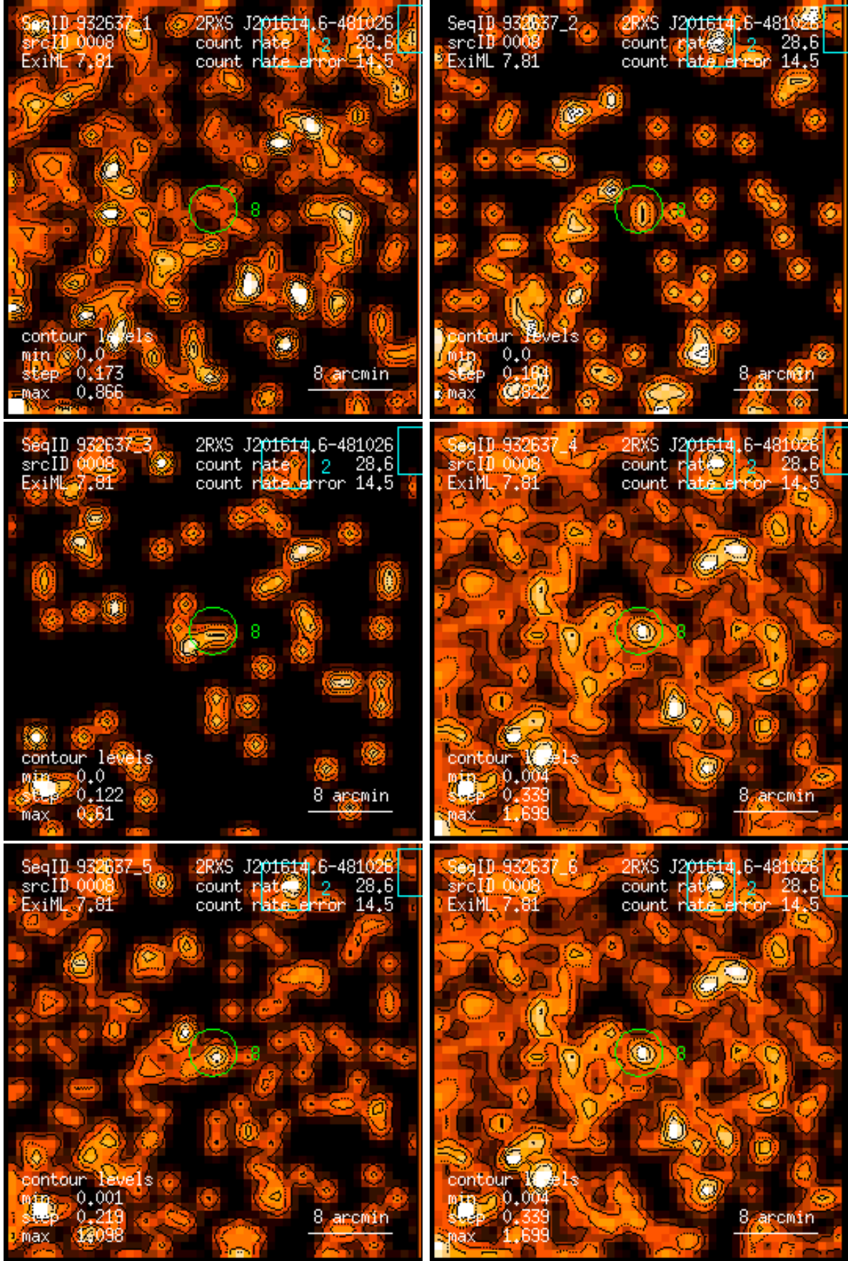
Figure 8: RASS 932637: detection 0008: band rate images, Gaussian filter: (1) PSPC channels 11 – 41, (2) 52 – 90, (3) 91 – 201, (4) 11 – 235, (5) 52 – 201, (6) 11 – 201. Broad band rates in counts/ks. Band rate contour levels in counts/ks/arcmin 2 .
