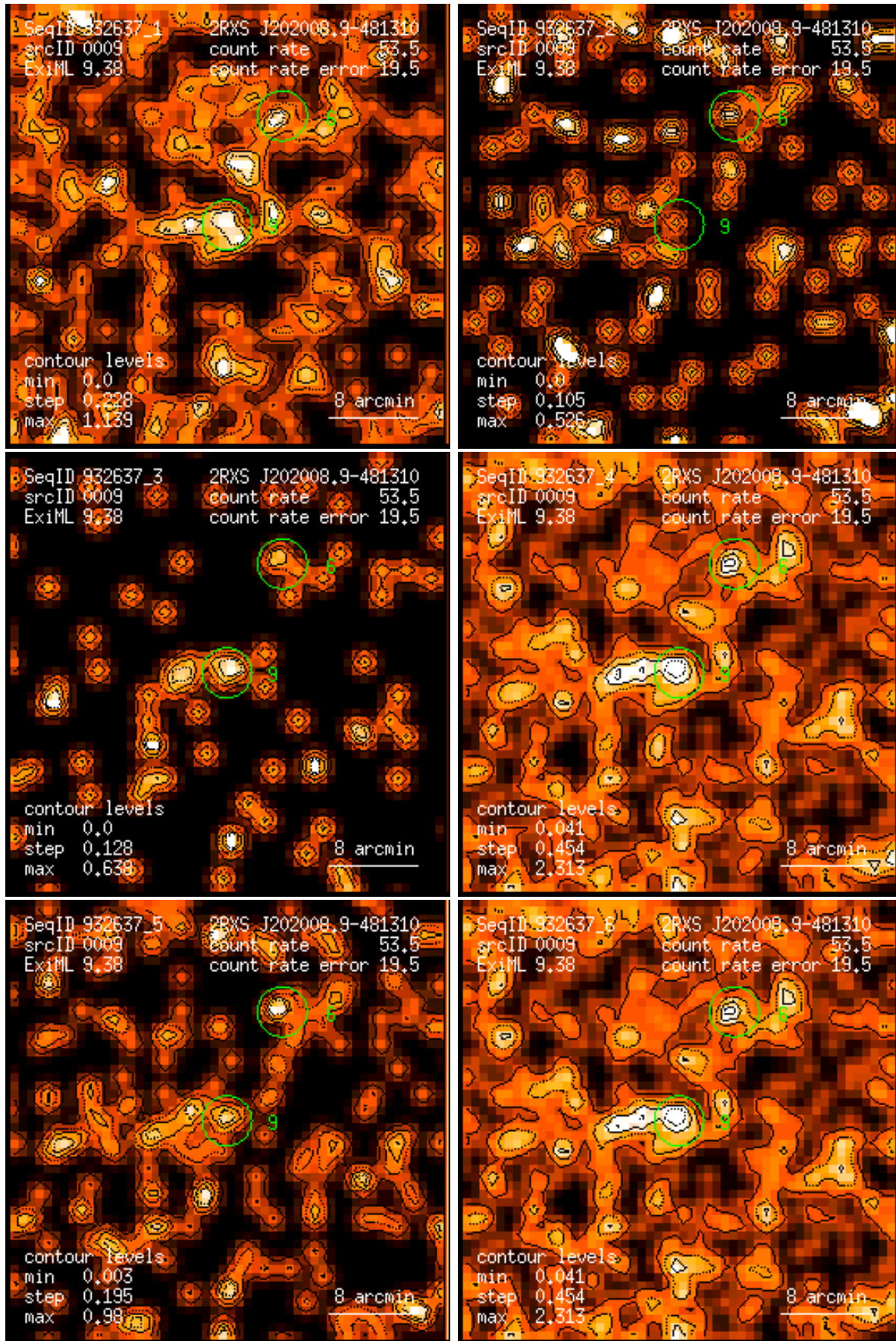
Figure 9: RASS 932637: detection 0009: band rate images, Gaussian filter: (1) PSPC channels 11 – 41, (2) 52 – 90, (3) 91 – 201, (4) 11 – 235, (5) 52 – 201, (6) 11 – 201. Broad band rates in counts/ks. Band rate contour levels in counts/ks/arcmin 2 .
