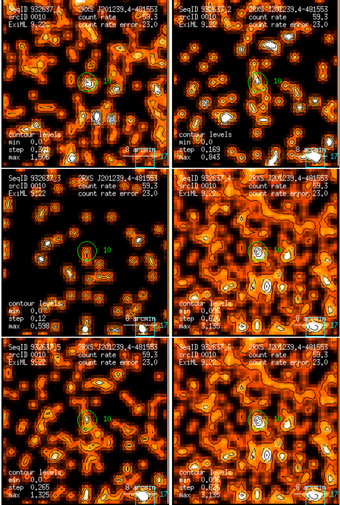
Figure 10: RASS 932637: detection 0010: band rate images, Gaussian filter: (1) PSPC channels 11 – 41, (2) 52 – 90, (3) 91 – 201, (4) 11 – 235, (5) 52 – 201, (6) 11 – 201. Broad band rates in counts/ks. Band rate contour levels in counts/ks/arcmin 2 .
