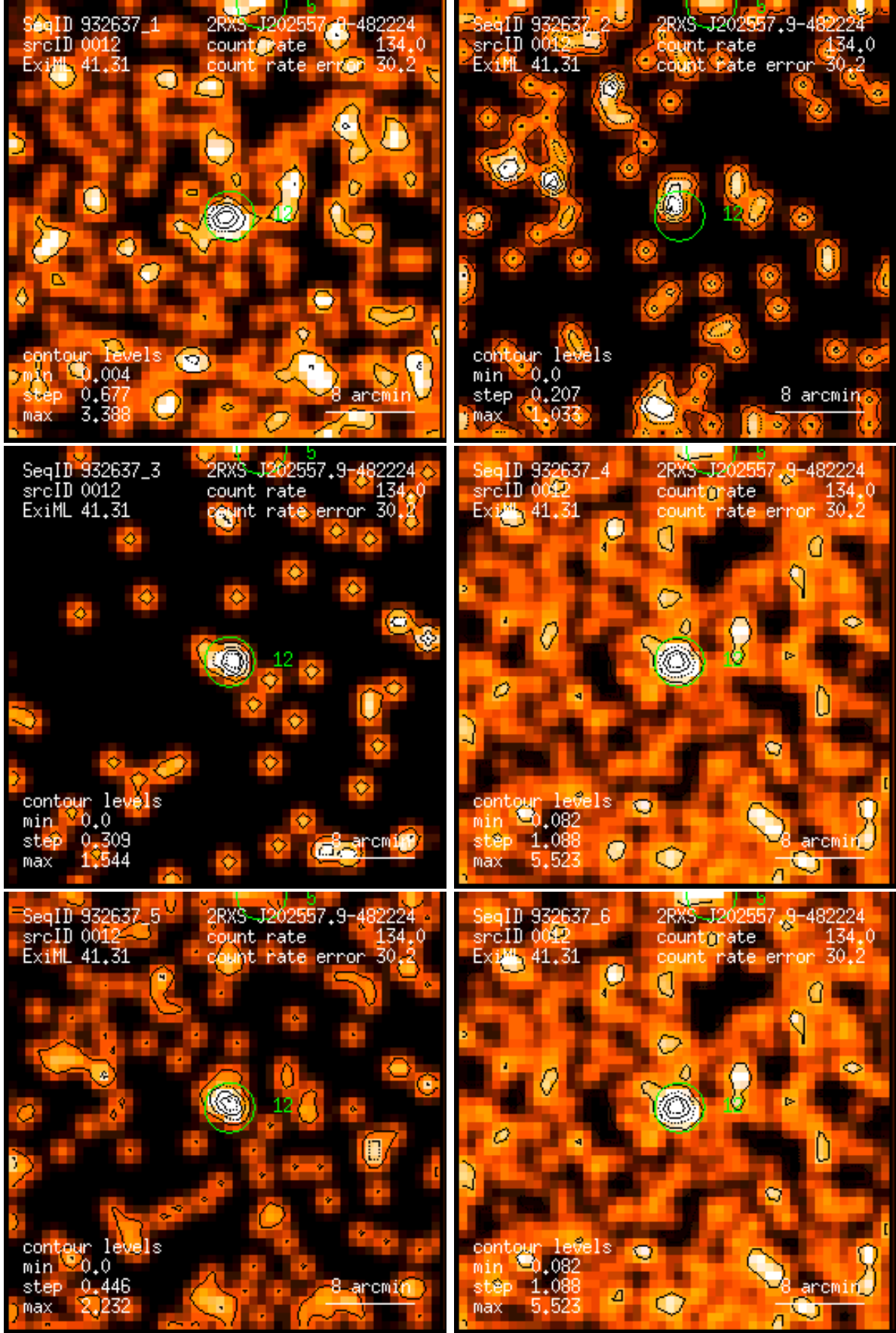
Figure 12: RASS 932637: detection 0012: band rate images, Gaussian filter: (1) PSPC channels 11 – 41, (2) 52 – 90, (3) 91 – 201, (4) 11 – 235, (5) 52 – 201, (6) 11 – 201. Broad band rates in counts/ks. Band rate contour levels in counts/ks/arcmin 2 .
