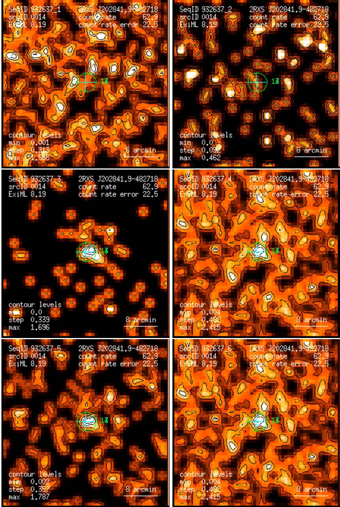
Figure 14: RASS 932637: detection 0014: band rate images, Gaussian filter: (1) PSPC channels 11 – 41, (2) 52 – 90, (3) 91 – 201, (4) 11 – 235, (5) 52 – 201, (6) 11 – 201. Broad band rates in counts/ks. Band rate contour levels in counts/ks/arcmin 2 .
