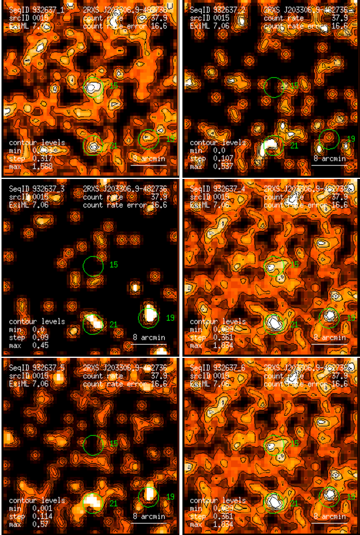
Figure 15: RASS 932637: detection 0015: band rate images, Gaussian filter: (1) PSPC channels 11 – 41, (2) 52 – 90, (3) 91 – 201, (4) 11 – 235, (5) 52 – 201, (6) 11 – 201. Broad band rates in counts/ks. Band rate contour levels in counts/ks/arcmin 2 .
