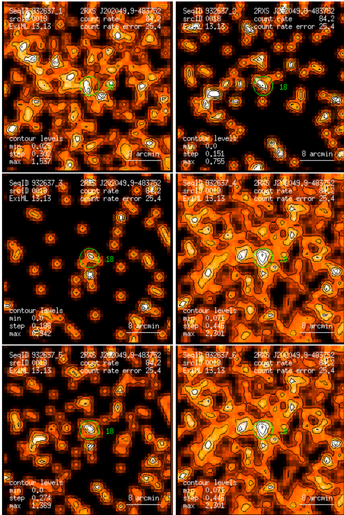
Figure 18: RASS 932637: detection 0018: band rate images, Gaussian filter: (1) PSPC channels 11 – 41, (2) 52 – 90, (3) 91 – 201, (4) 11 – 235, (5) 52 – 201, (6) 11 – 201. Broad band rates in counts/ks. Band rate contour levels in counts/ks/arcmin 2 .
