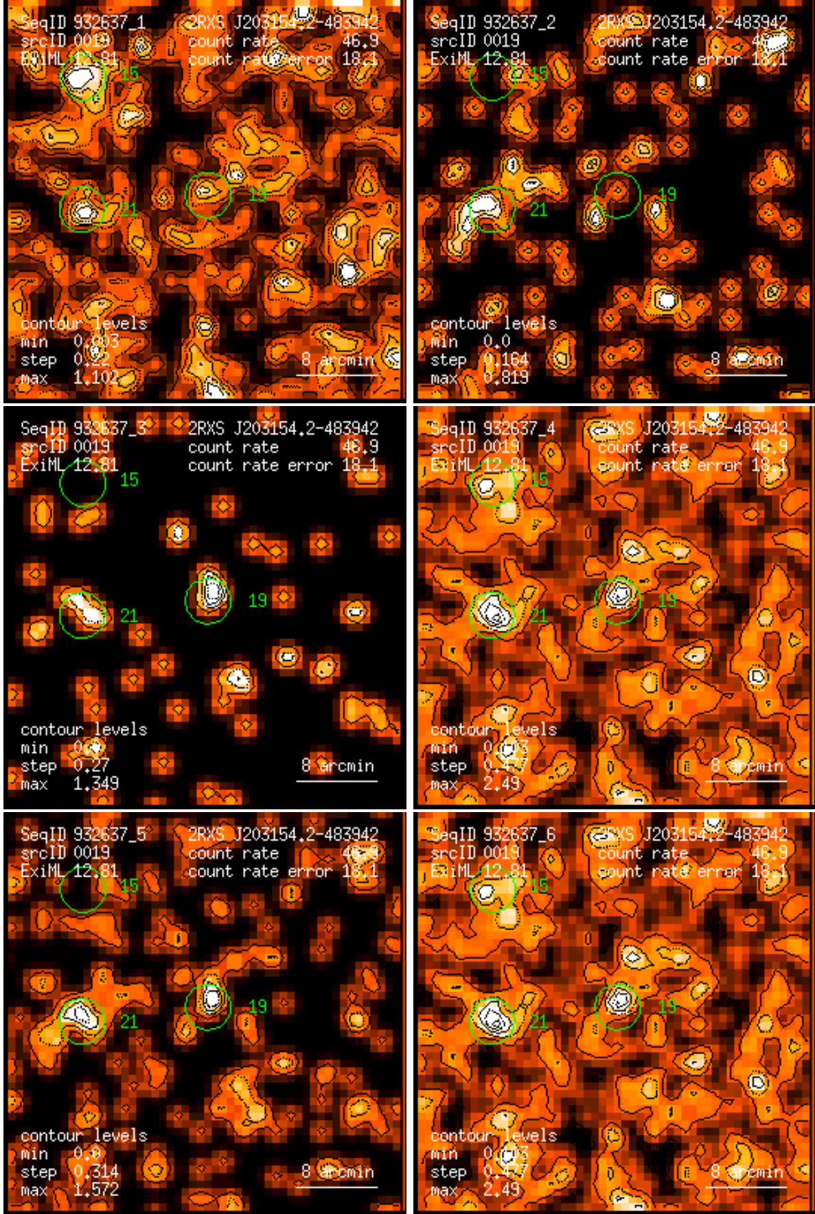
Figure 19: RASS 932637: detection 0019: band rate images, Gaussian filter: (1) PSPC channels 11 – 41, (2) 52 – 90, (3) 91 – 201, (4) 11 – 235, (5) 52 – 201, (6) 11 – 201. Broad band rates in counts/ks. Band rate contour levels in counts/ks/arcmin 2 .
