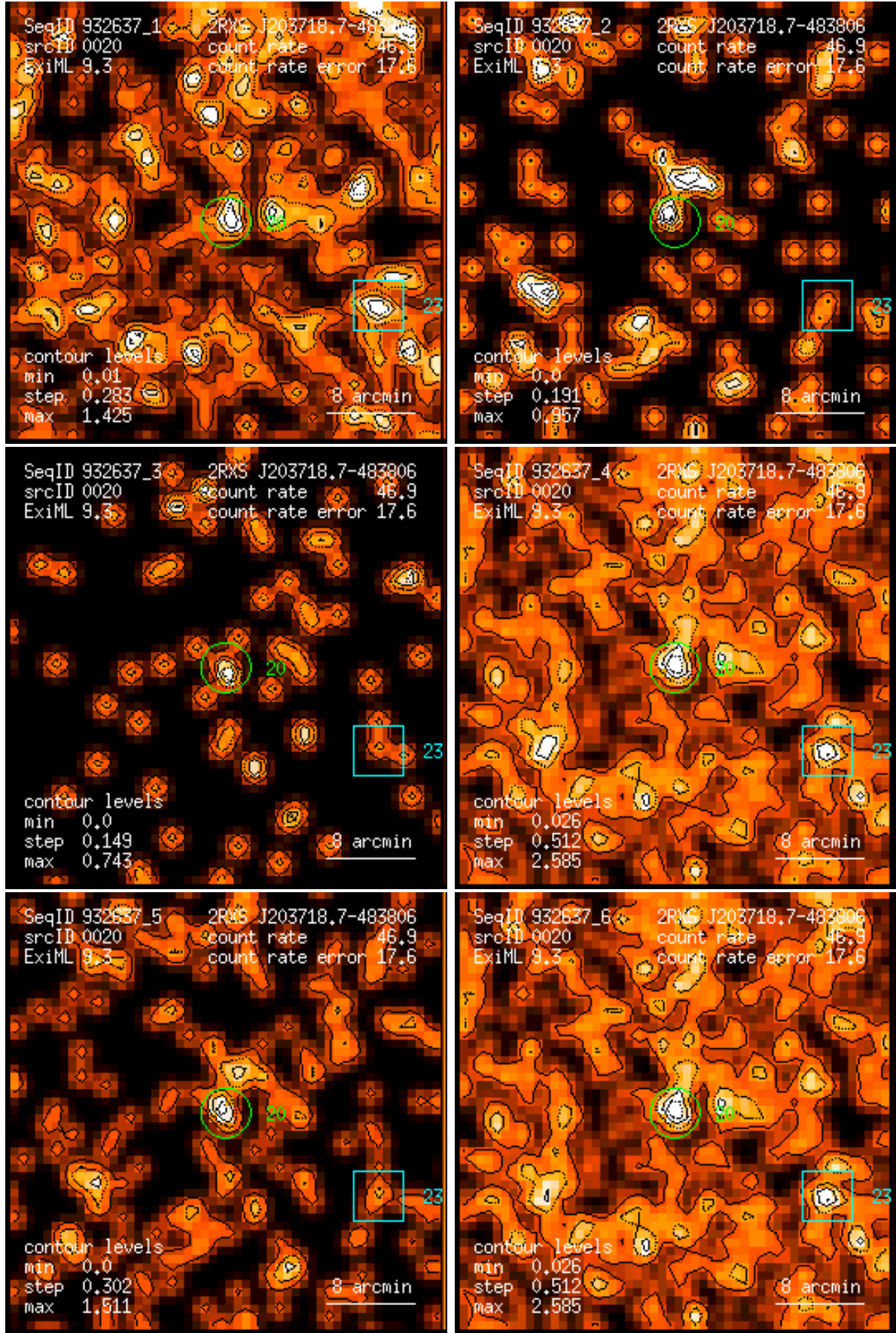
Figure 20: RASS 932637: detection 0020: band rate images, Gaussian filter: (1) PSPC channels 11 – 41, (2) 52 – 90, (3) 91 – 201, (4) 11 – 235, (5) 52 – 201, (6) 11 – 201. Broad band rates in counts/ks. Band rate contour levels in counts/ks/arcmin 2 .
