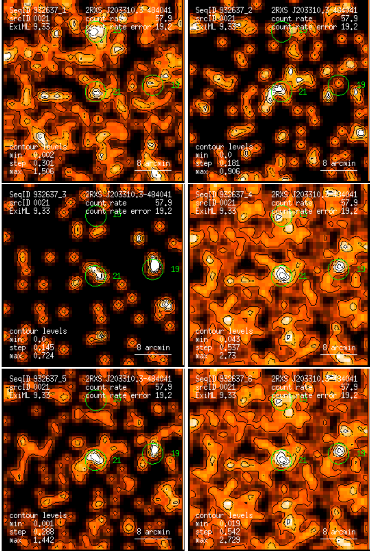
Figure 21: RASS 932637: detection 0021: band rate images, Gaussian filter: (1) PSPC channels 11 – 41, (2) 52 – 90, (3) 91 – 201, (4) 11 – 235, (5) 52 – 201, (6) 11 – 201. Broad band rates in counts/ks. Band rate contour levels in counts/ks/arcmin 2 .
