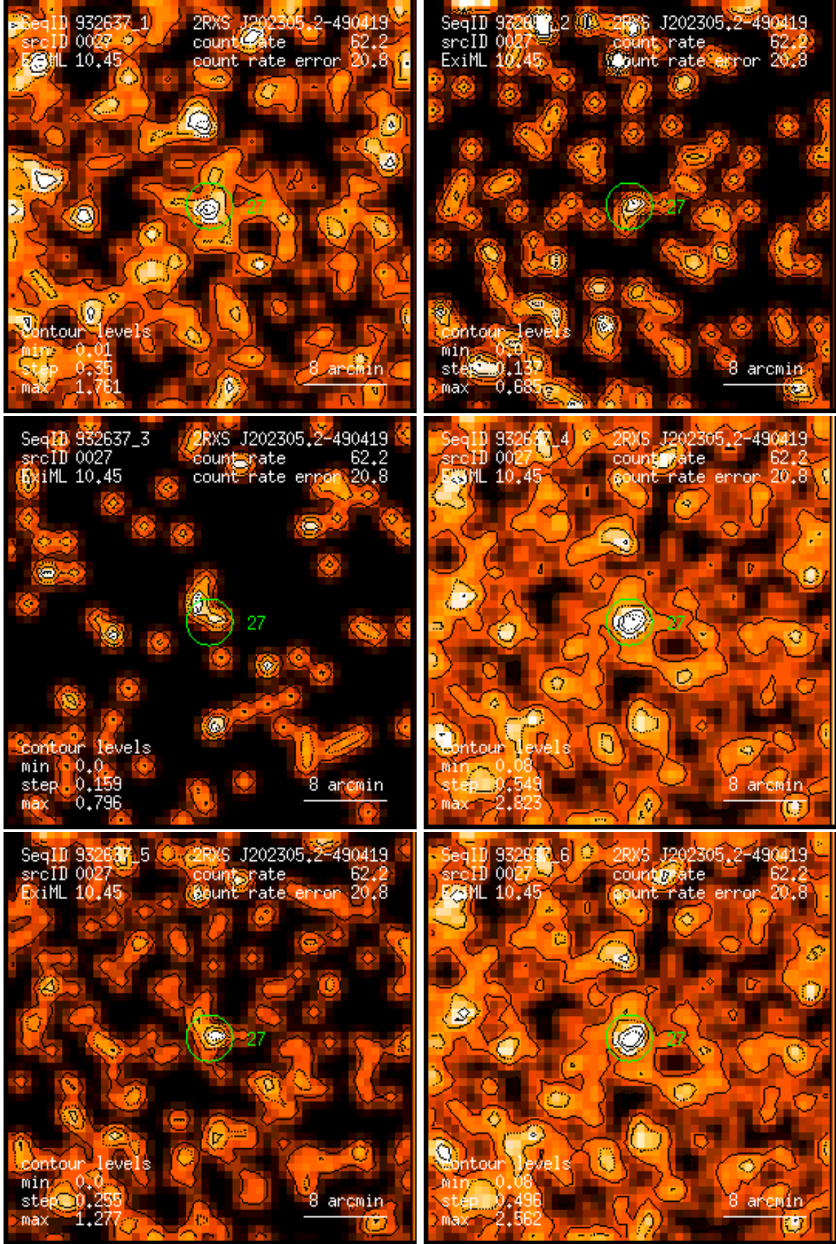
Figure 27: RASS 932637: detection 0027: band rate images, Gaussian filter: (1) PSPC channels 11 – 41, (2) 52 – 90, (3) 91 – 201, (4) 11 – 235, (5) 52 – 201, (6) 11 – 201. Broad band rates in counts/ks. Band rate contour levels in counts/ks/arcmin 2 .
