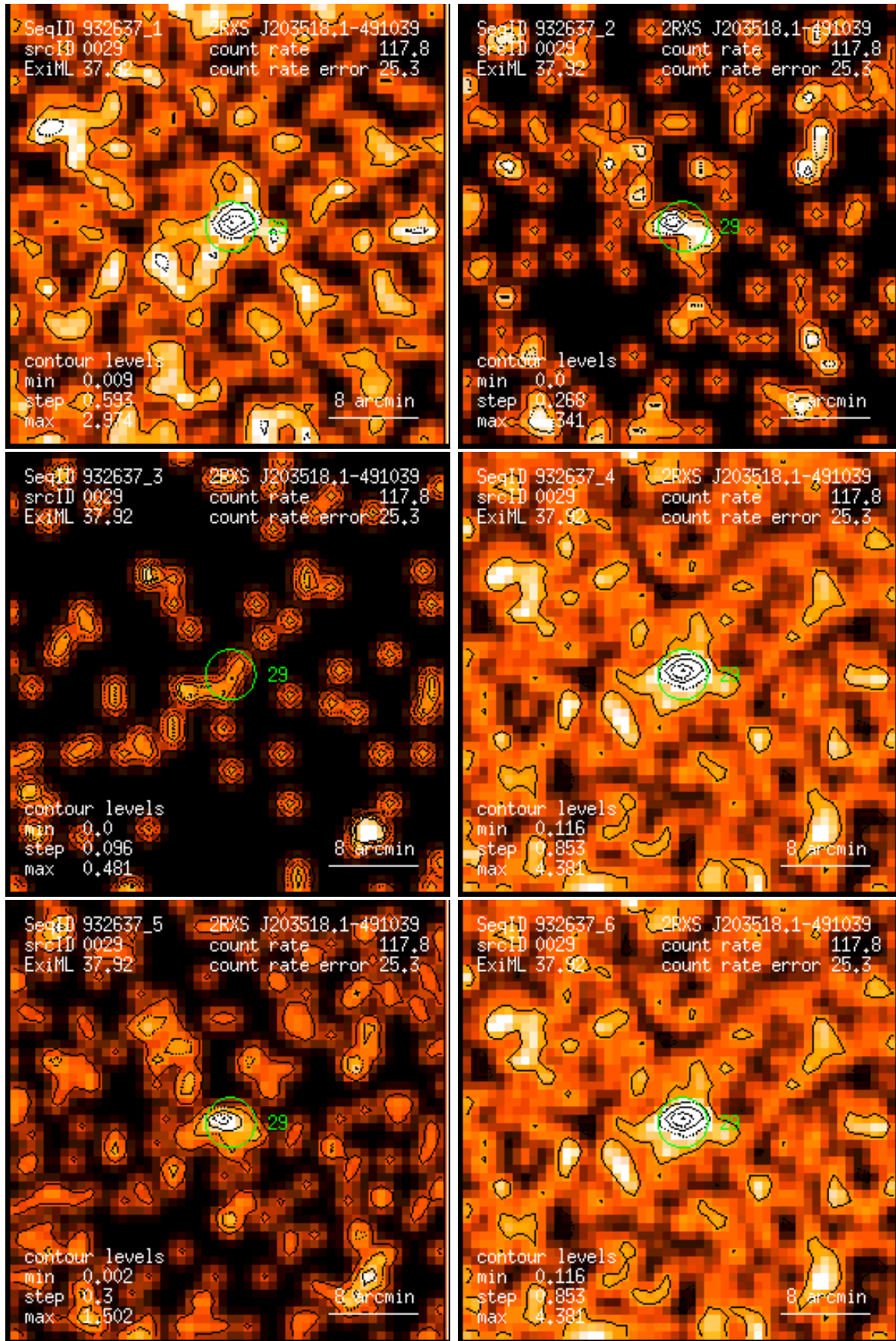
Figure 29: RASS 932637: detection 0029: band rate images, Gaussian filter: (1) PSPC channels 11 – 41, (2) 52 – 90, (3) 91 – 201, (4) 11 – 235, (5) 52 – 201, (6) 11 – 201. Broad band rates in counts/ks. Band rate contour levels in counts/ks/arcmin 2 .
