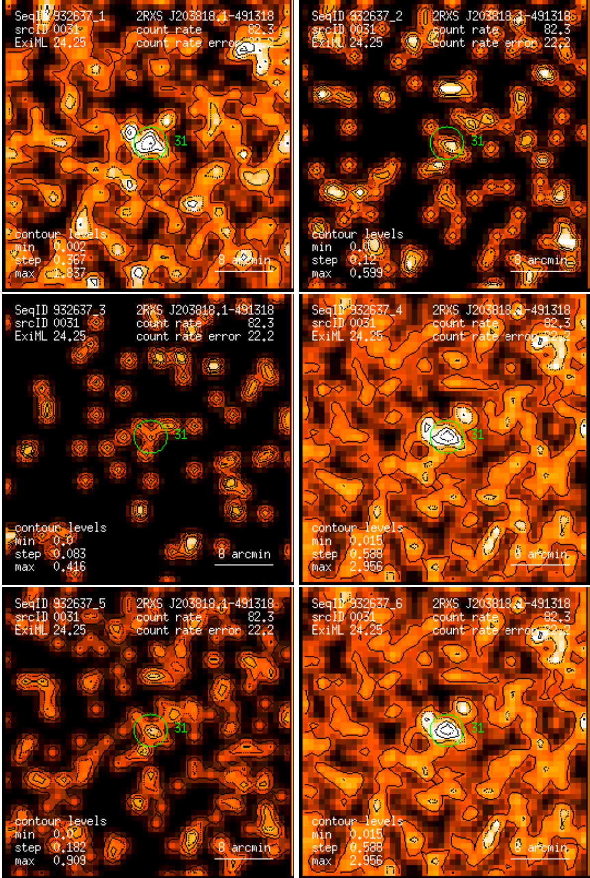
Figure 31: RASS 932637: detection 0031: band rate images, Gaussian filter: (1) PSPC channels 11 – 41, (2) 52 – 90, (3) 91 – 201, (4) 11 – 235, (5) 52 – 201, (6) 11 – 201. Broad band rates in counts/ks. Band rate contour levels in counts/ks/arcmin 2 .
