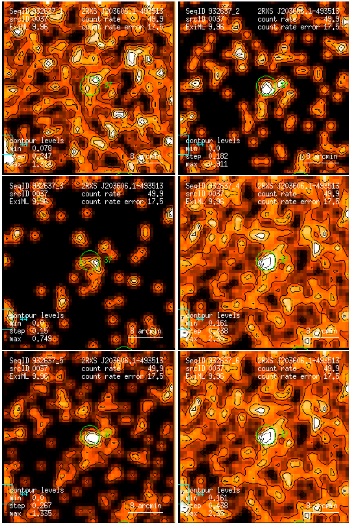
Figure 37: RASS 932637: detection 0037: band rate images, Gaussian filter: (1) PSPC channels 11 – 41, (2) 52 – 90, (3) 91 – 201, (4) 11 – 235, (5) 52 – 201, (6) 11 – 201. Broad band rates in counts/ks. Band rate contour levels in counts/ks/arcmin 2 .
