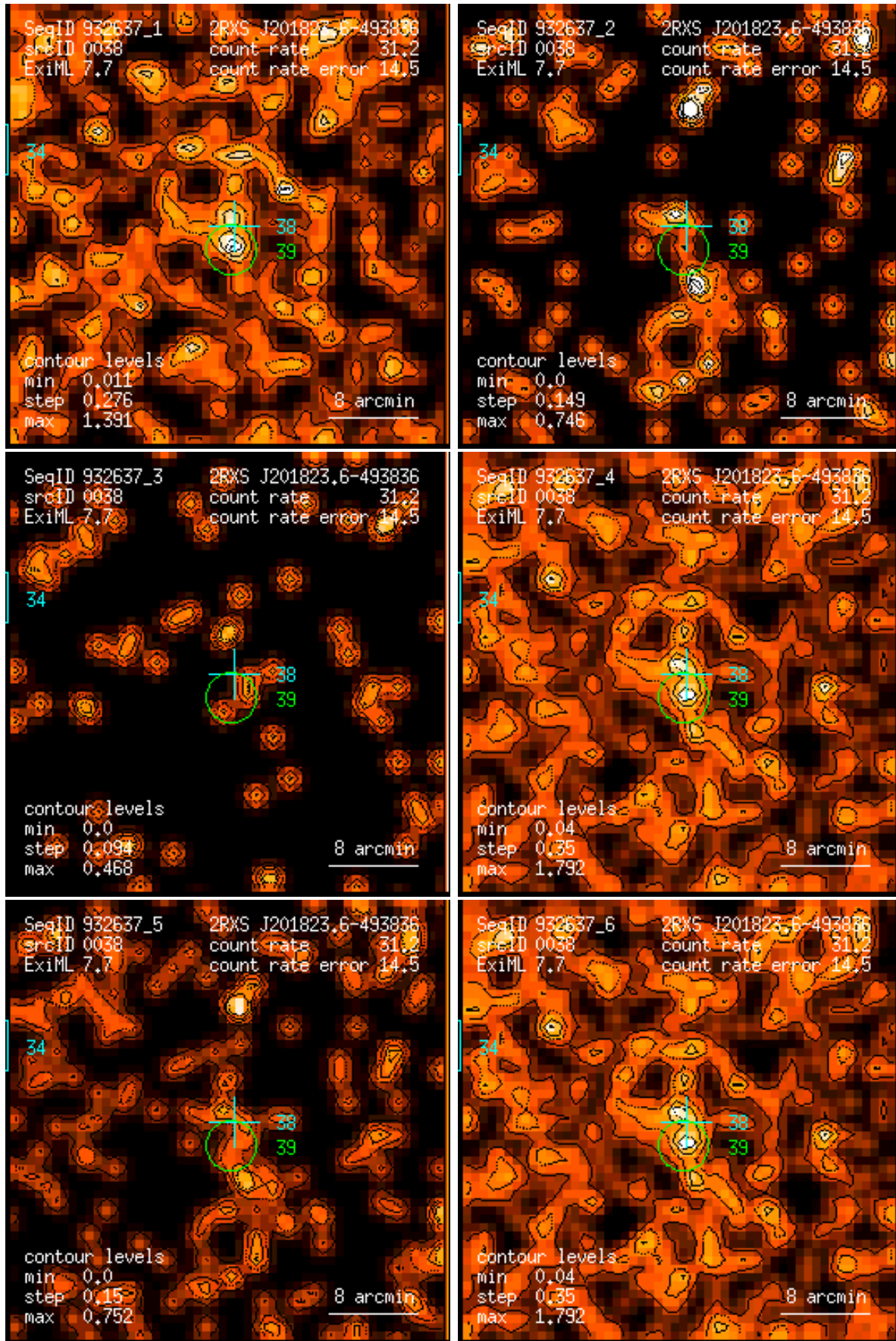
Figure 38: RASS 932637: detection 0038: band rate images, Gaussian filter: (1) PSPC channels 11 – 41, (2) 52 – 90, (3) 91 – 201, (4) 11 – 235, (5) 52 – 201, (6) 11 – 201. Broad band rates in counts/ks. Band rate contour levels in counts/ks/arcmin 2 .
