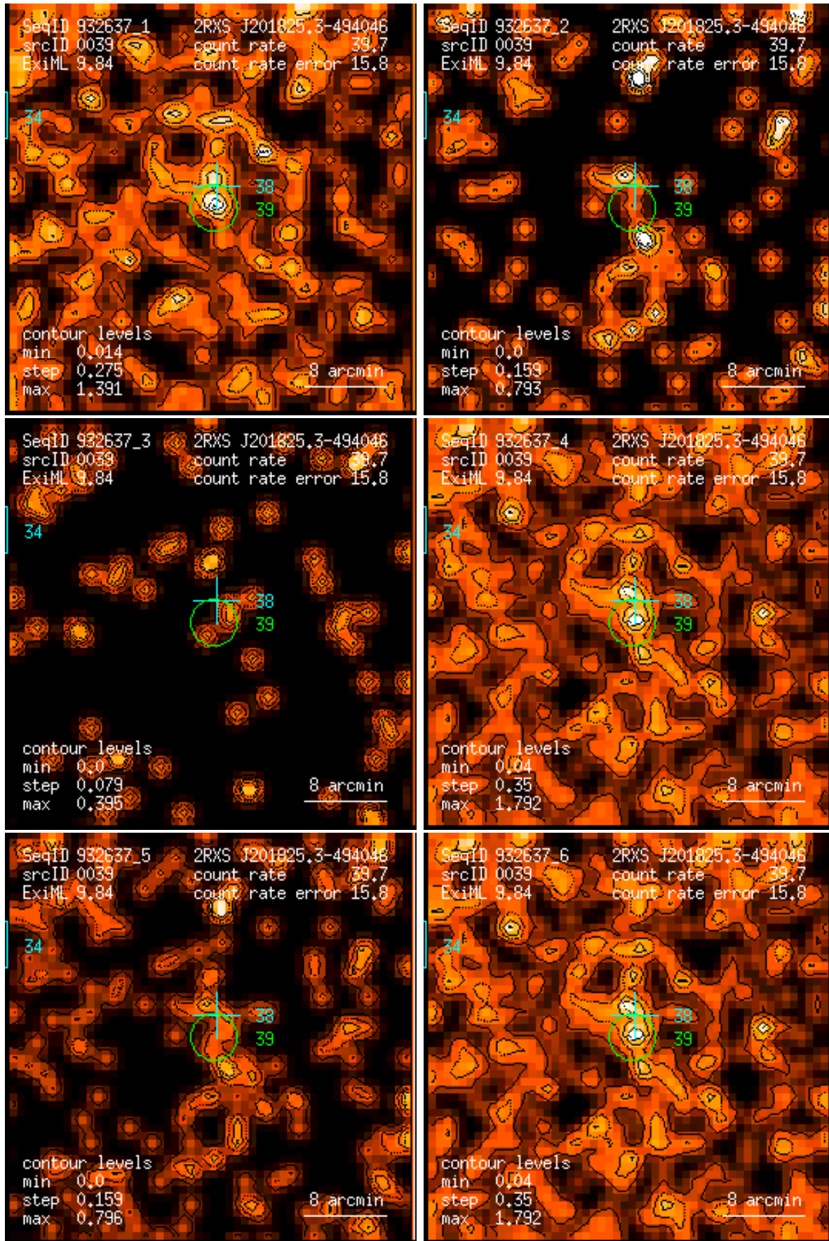
Figure 39: RASS 932637: detection 0039: band rate images, Gaussian filter: (1) PSPC channels 11 – 41, (2) 52 – 90, (3) 91 – 201, (4) 11 – 235, (5) 52 – 201, (6) 11 – 201. Broad band rates in counts/ks. Band rate contour levels in counts/ks/arcmin 2 .
