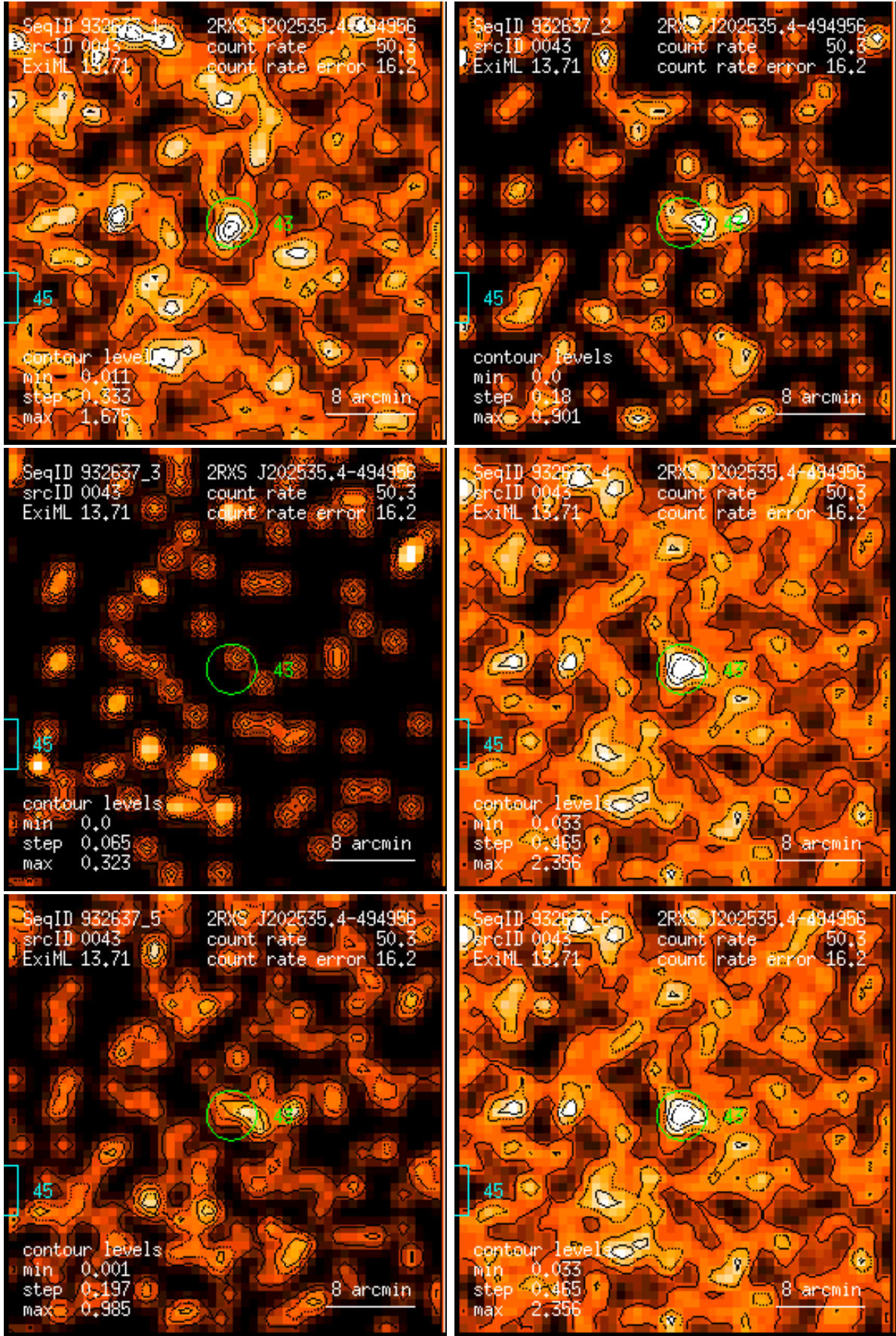
Figure 43: RASS 932637: detection 0043: band rate images, Gaussian filter: (1) PSPC channels 11 – 41, (2) 52 – 90, (3) 91 – 201, (4) 11 – 235, (5) 52 – 201, (6) 11 – 201. Broad band rates in counts/ks. Band rate contour levels in counts/ks/arcmin 2 .
