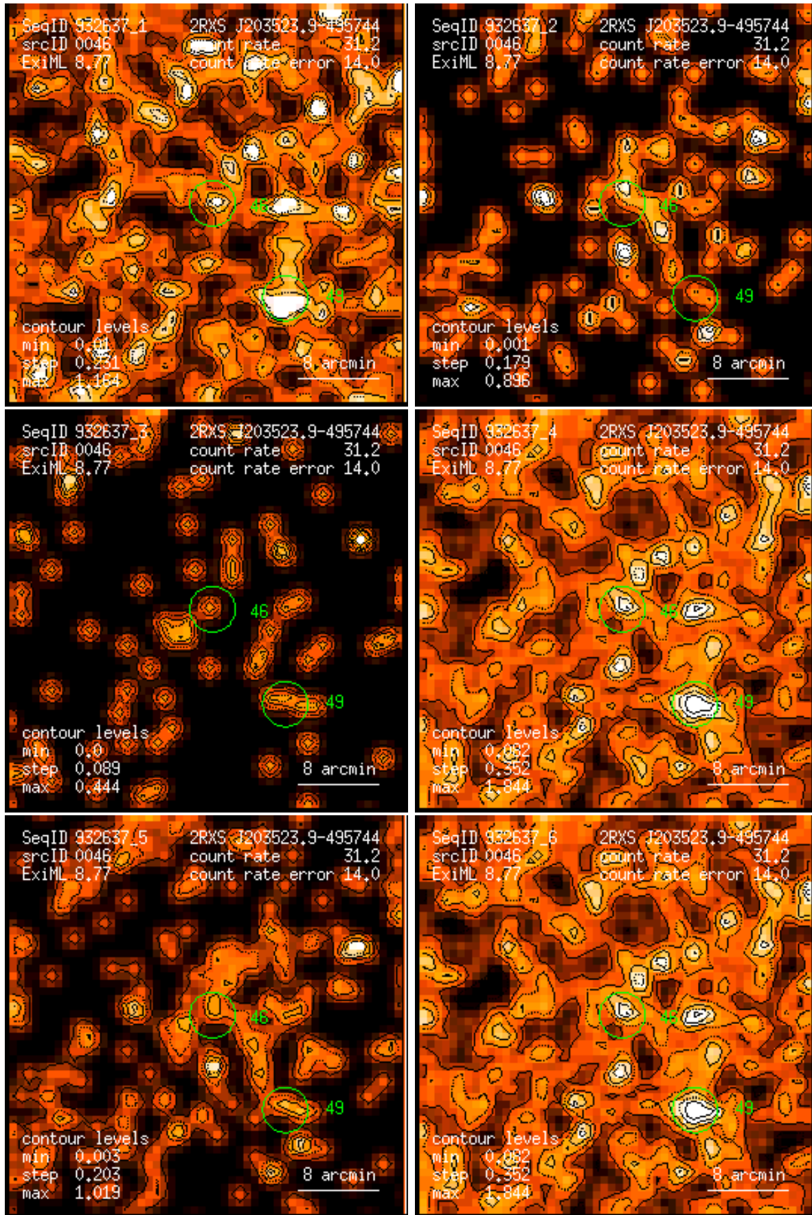
Figure 46: RASS 932637: detection 0046: band rate images, Gaussian filter: (1) PSPC channels 11 – 41, (2) 52 – 90, (3) 91 – 201, (4) 11 – 235, (5) 52 – 201, (6) 11 – 201. Broad band rates in counts/ks. Band rate contour levels in counts/ks/arcmin 2 .
