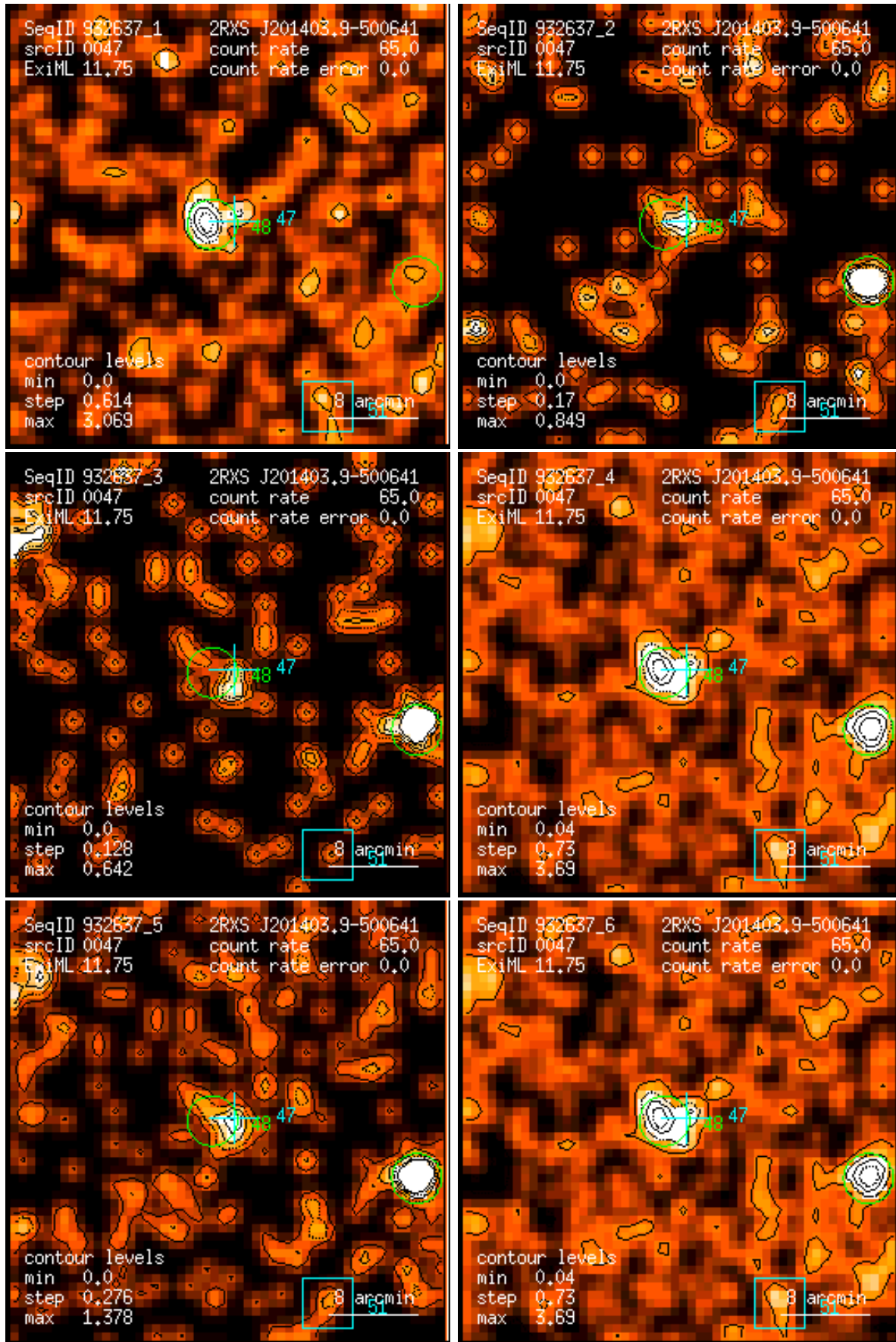
Figure 47: RASS 932637: detection 0047: band rate images, Gaussian filter: (1) PSPC channels 11 – 41, (2) 52 – 90, (3) 91 – 201, (4) 11 – 235, (5) 52 – 201, (6) 11 – 201. Broad band rates in counts/ks. Band rate contour levels in counts/ks/arcmin 2 .
