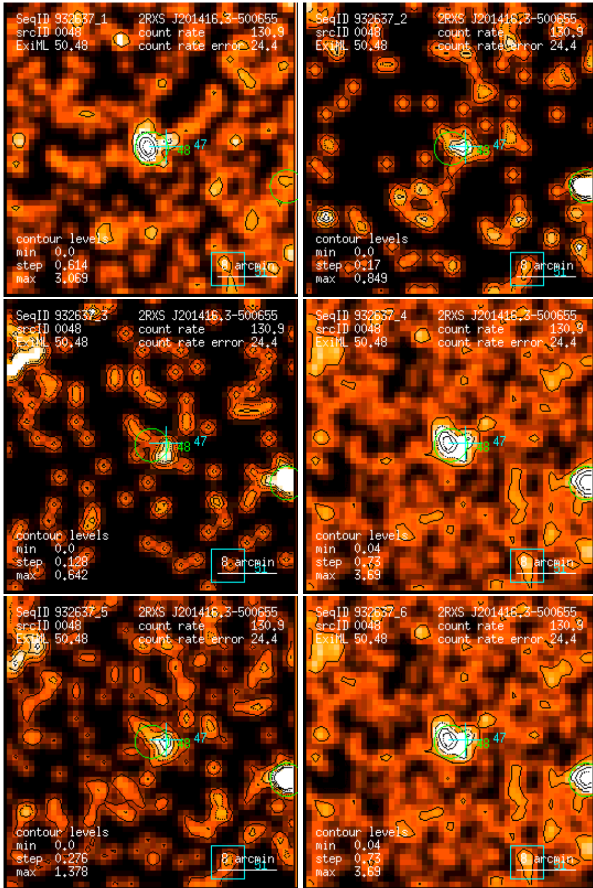
Figure 48: RASS 932637: detection 0048: band rate images, Gaussian filter: (1) PSPC channels 11 – 41, (2) 52 – 90, (3) 91 – 201, (4) 11 – 235, (5) 52 – 201, (6) 11 – 201. Broad band rates in counts/ks. Band rate contour levels in counts/ks/arcmin 2 .
