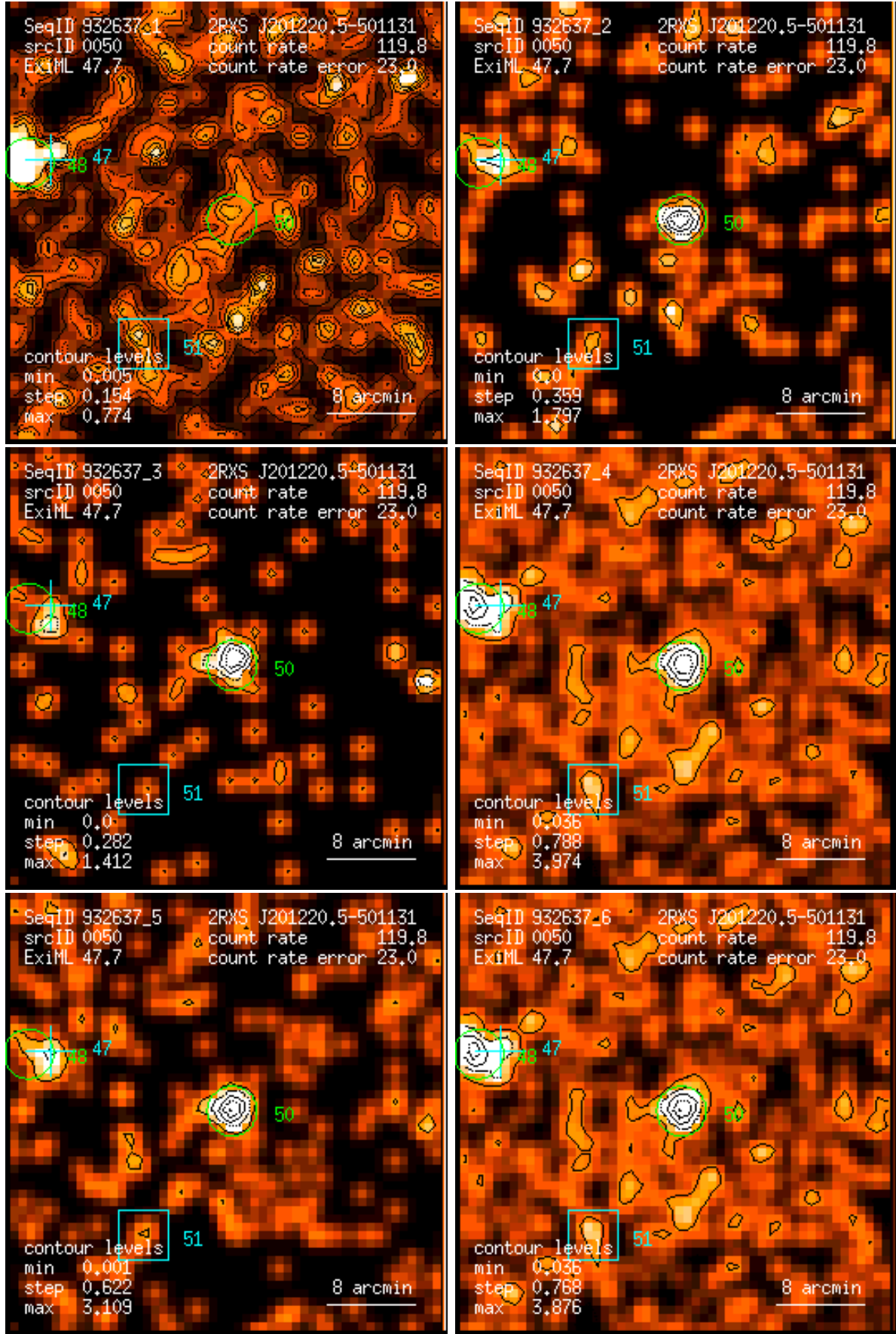
Figure 50: RASS 932637: detection 0050: band rate images, Gaussian filter: (1) PSPC channels 11 – 41, (2) 52 – 90, (3) 91 – 201, (4) 11 – 235, (5) 52 – 201, (6) 11 – 201. Broad band rates in counts/ks. Band rate contour levels in counts/ks/arcmin 2 .
