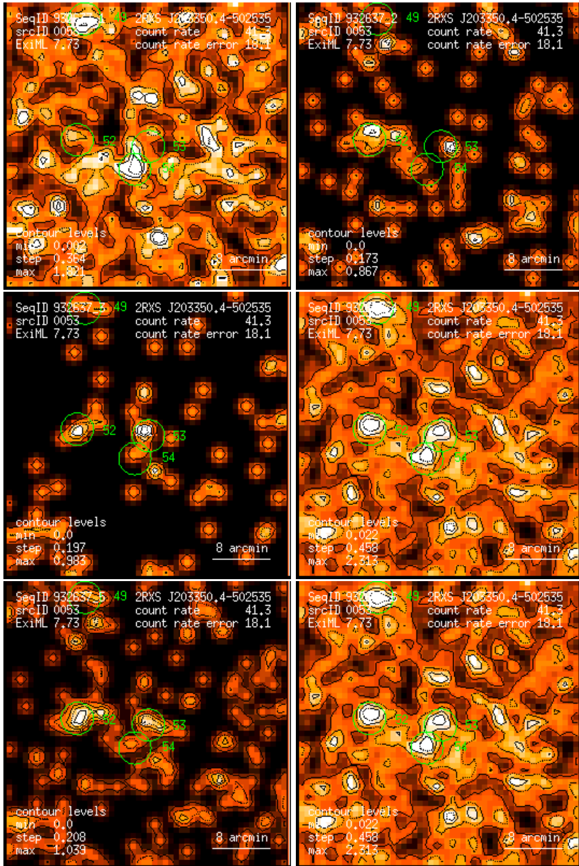
Figure 53: RASS 932637: detection 0053: band rate images, Gaussian filter: (1) PSPC channels 11 – 41, (2) 52 – 90, (3) 91 – 201, (4) 11 – 235, (5) 52 – 201, (6) 11 – 201. Broad band rates in counts/ks. Band rate contour levels in counts/ks/arcmin 2 .
