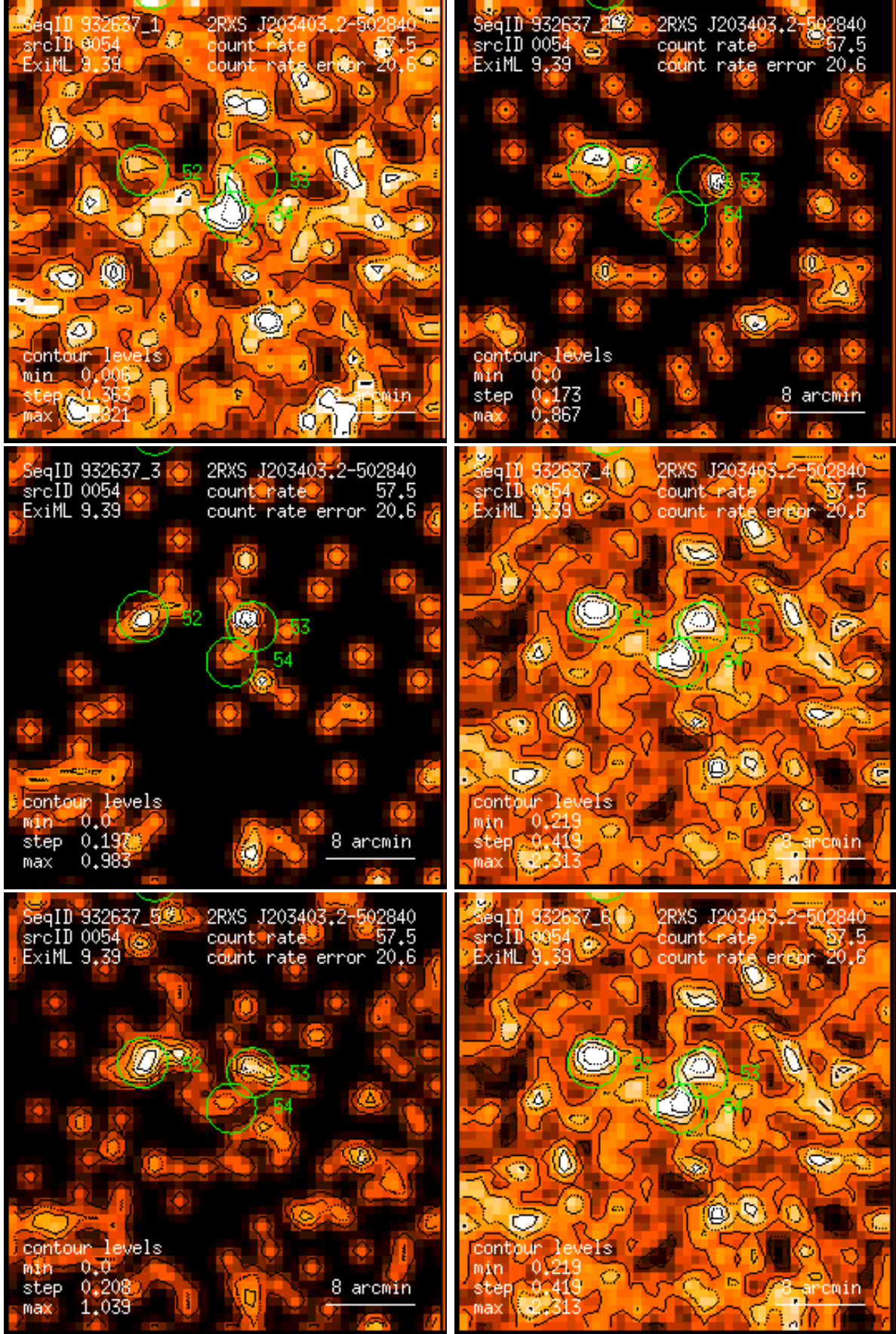
Figure 54: RASS 932637: detection 0054: band rate images, Gaussian filter: (1) PSPC channels 11 – 41, (2) 52 – 90, (3) 91 – 201, (4) 11 – 235, (5) 52 – 201, (6) 11 – 201. Broad band rates in counts/ks. Band rate contour levels in counts/ks/arcmin 2 .
