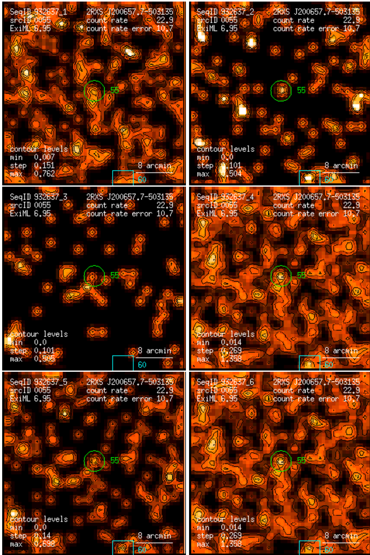
Figure 55: RASS 932637: detection 0055: band rate images, Gaussian filter: (1) PSPC channels 11 – 41, (2) 52 – 90, (3) 91 – 201, (4) 11 – 235, (5) 52 – 201, (6) 11 – 201. Broad band rates in counts/ks. Band rate contour levels in counts/ks/arcmin 2 .
