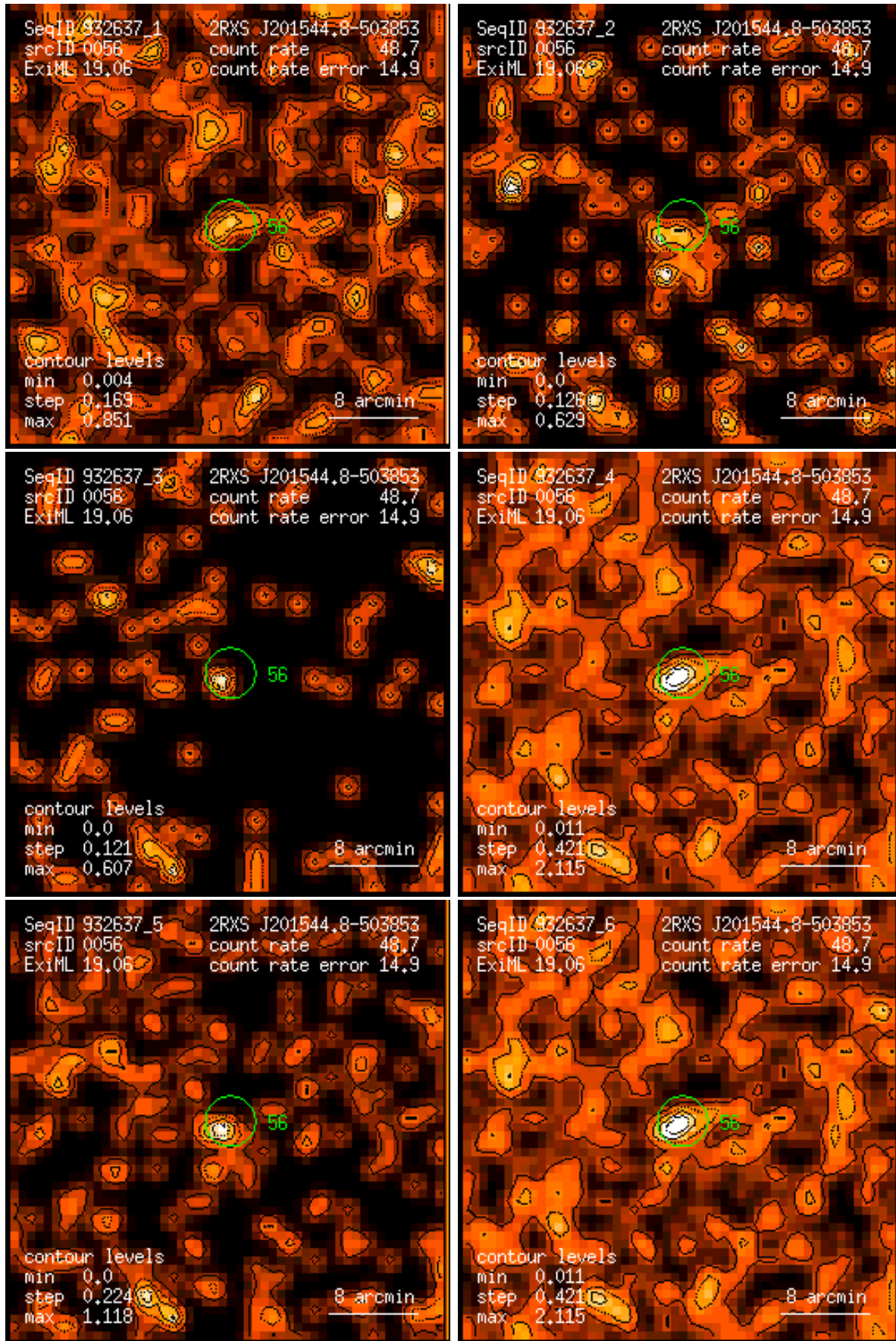
Figure 56: RASS 932637: detection 0056: band rate images, Gaussian filter: (1) PSPC channels 11 – 41, (2) 52 – 90, (3) 91 – 201, (4) 11 – 235, (5) 52 – 201, (6) 11 – 201. Broad band rates in counts/ks. Band rate contour levels in counts/ks/arcmin 2 .
