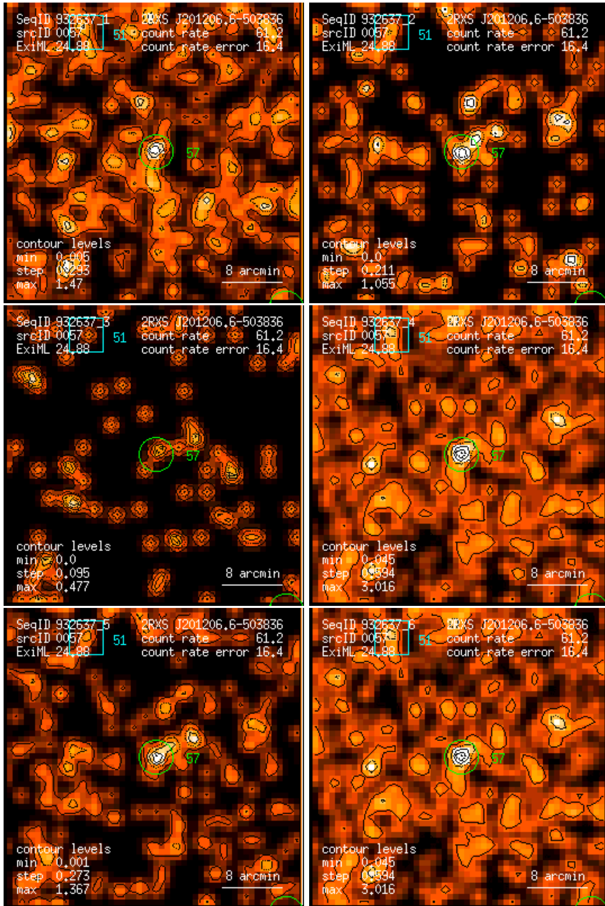
Figure 57: RASS 932637: detection 0057: band rate images, Gaussian filter: (1) PSPC channels 11 – 41, (2) 52 – 90, (3) 91 – 201, (4) 11 – 235, (5) 52 – 201, (6) 11 – 201. Broad band rates in counts/ks. Band rate contour levels in counts/ks/arcmin 2 .
