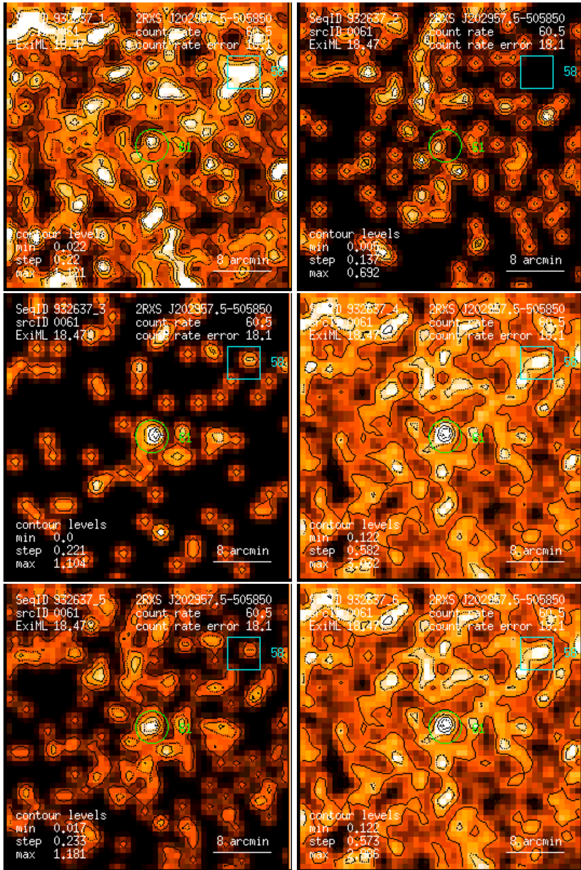
Figure 61: RASS 932637: detection 0061: band rate images, Gaussian filter: (1) PSPC channels 11 – 41, (2) 52 – 90, (3) 91 – 201, (4) 11 – 235, (5) 52 – 201, (6) 11 – 201. Broad band rates in counts/ks. Band rate contour levels in counts/ks/arcmin 2 .
