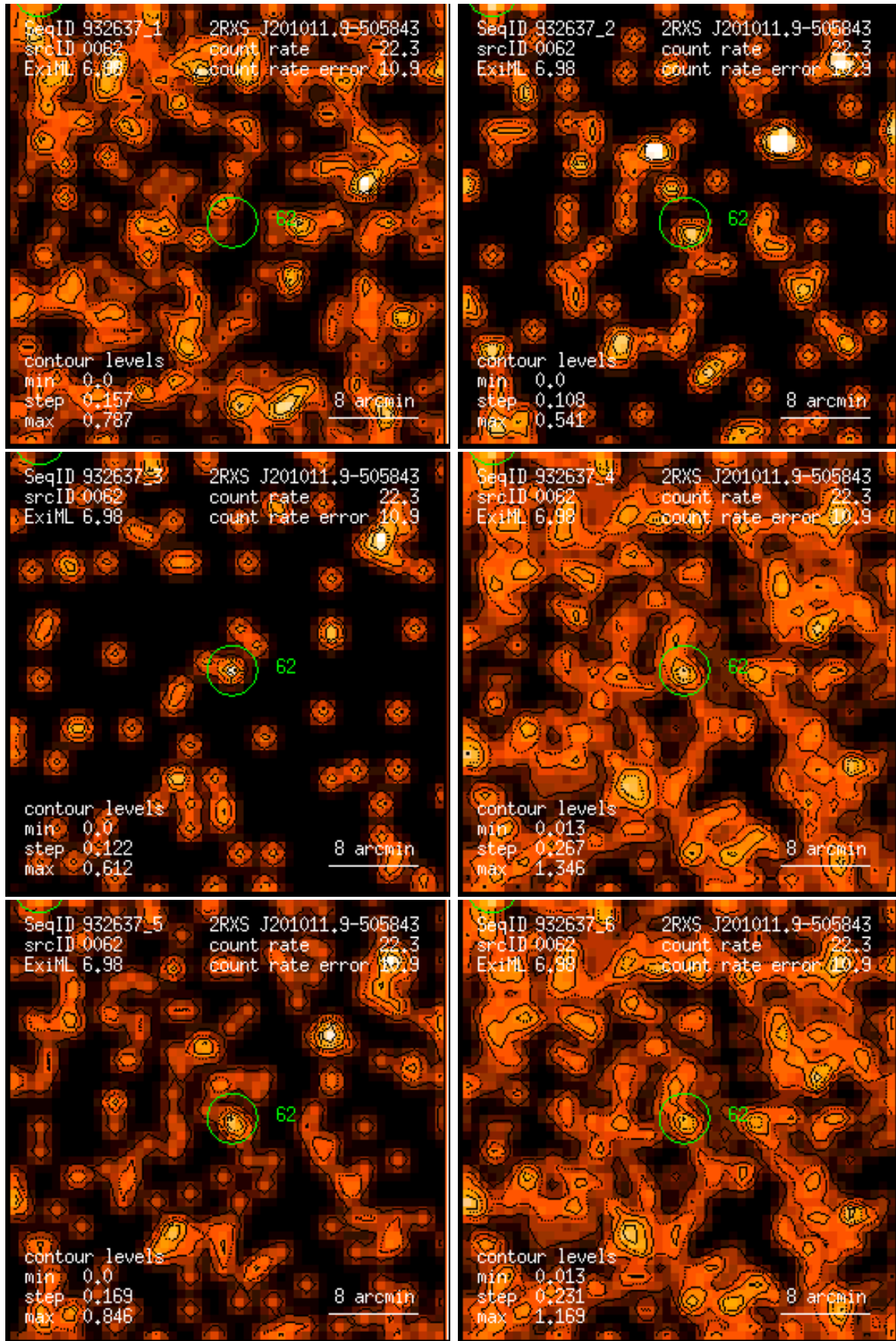
Figure 62: RASS 932637: detection 0062: band rate images, Gaussian filter: (1) PSPC channels 11 – 41, (2) 52 – 90, (3) 91 – 201, (4) 11 – 235, (5) 52 – 201, (6) 11 – 201. Broad band rates in counts/ks. Band rate contour levels in counts/ks/arcmin 2 .
