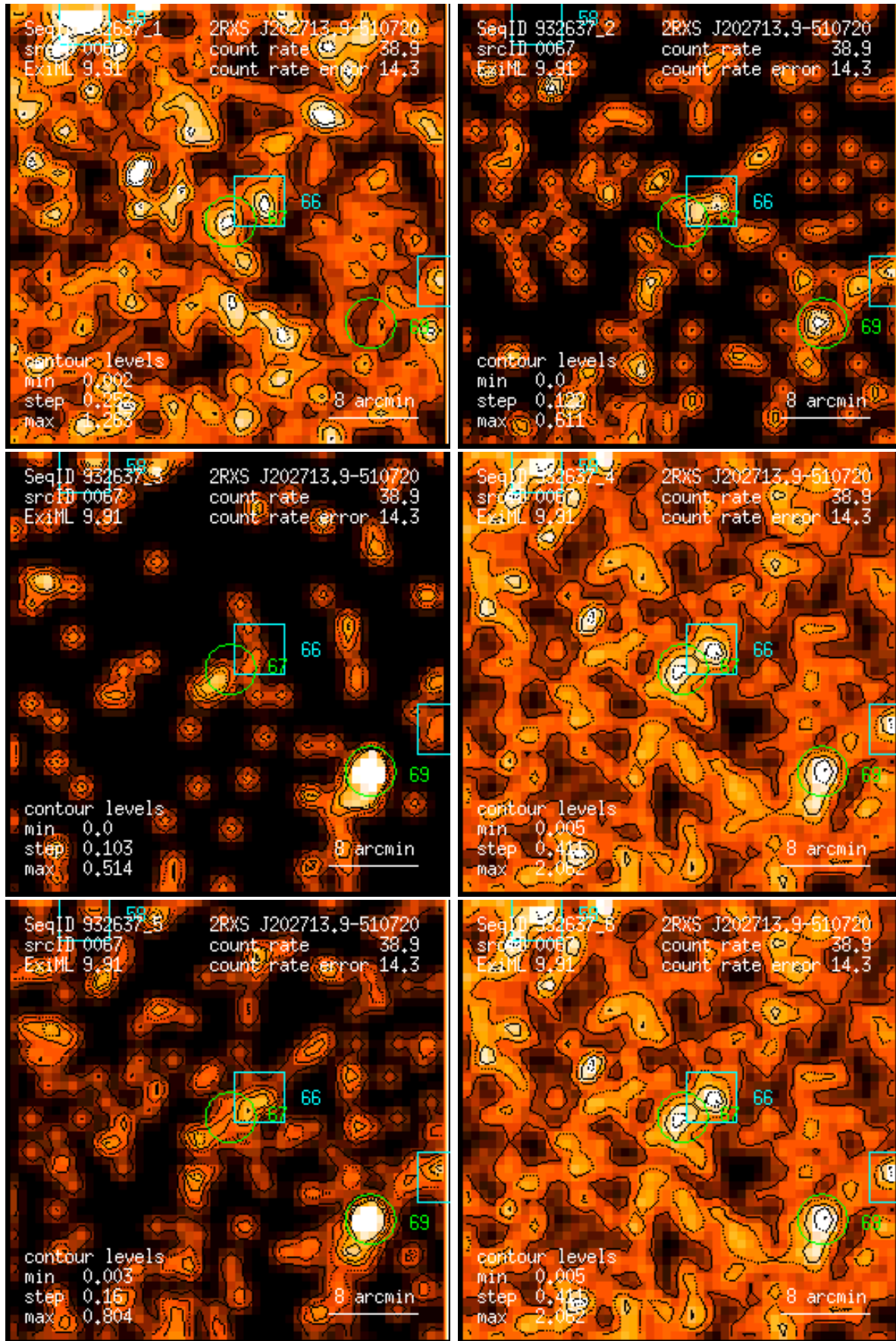
Figure 67: RASS 932637: detection 0067: band rate images, Gaussian filter: (1) PSPC channels 11 – 41, (2) 52 – 90, (3) 91 – 201, (4) 11 – 235, (5) 52 – 201, (6) 11 – 201. Broad band rates in counts/ks. Band rate contour levels in counts/ks/arcmin 2 .
