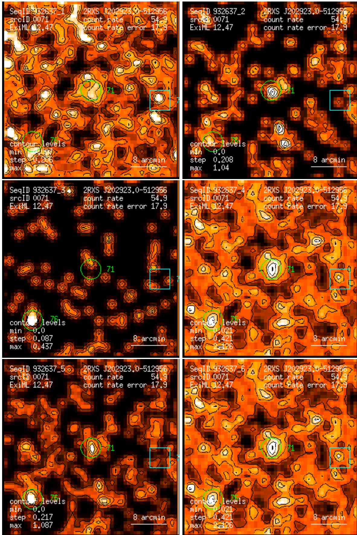
Figure 71: RASS 932637: detection 0071: band rate images, Gaussian filter: (1) PSPC channels 11 – 41, (2) 52 – 90, (3) 91 – 201, (4) 11 – 235, (5) 52 – 201, (6) 11 – 201. Broad band rates in counts/ks. Band rate contour levels in counts/ks/arcmin 2 .
