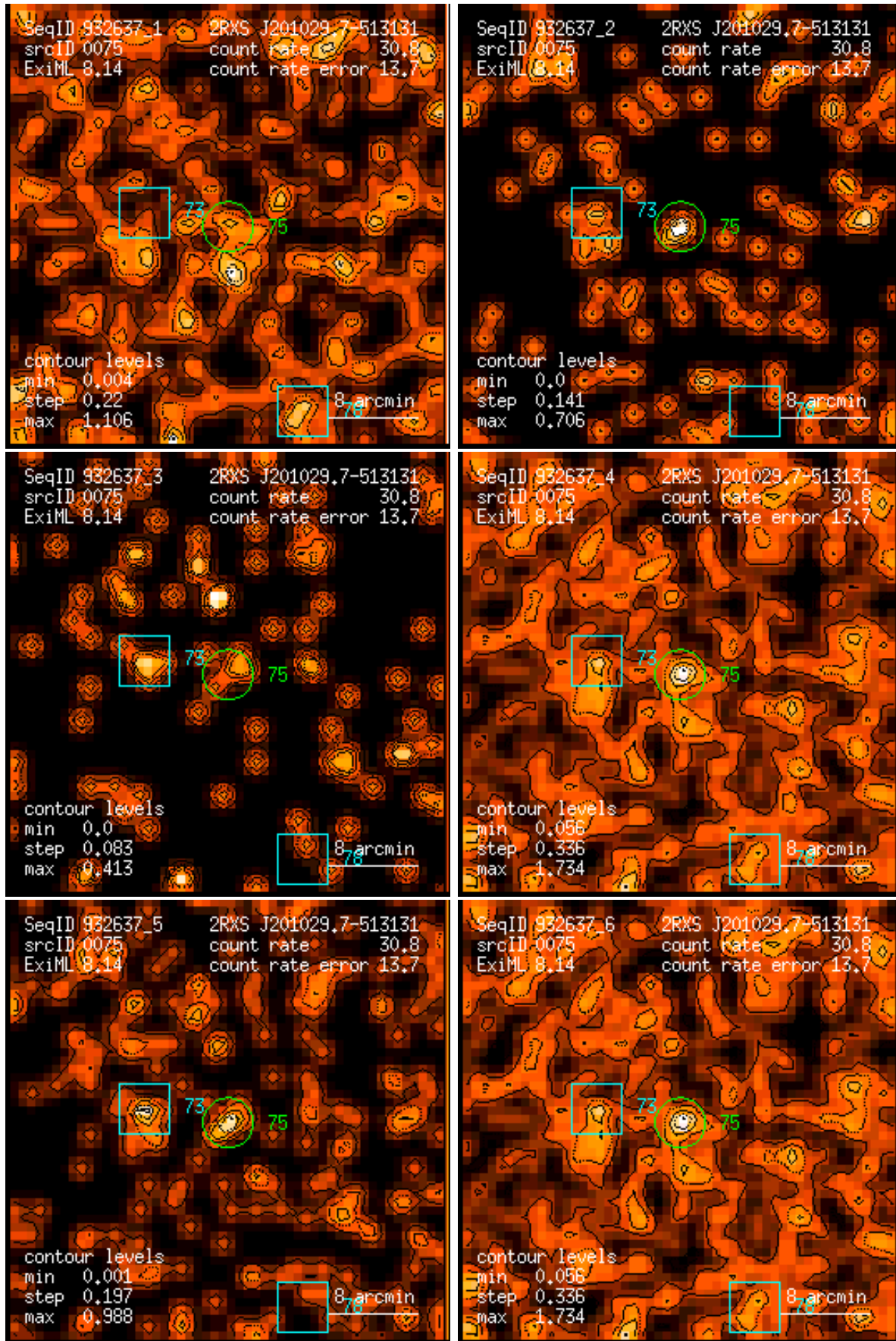
Figure 75: RASS 932637: detection 0075: band rate images, Gaussian filter: (1) PSPC channels 11 – 41, (2) 52 – 90, (3) 91 – 201, (4) 11 – 235, (5) 52 – 201, (6) 11 – 201. Broad band rates in counts/ks. Band rate contour levels in counts/ks/arcmin 2 .
