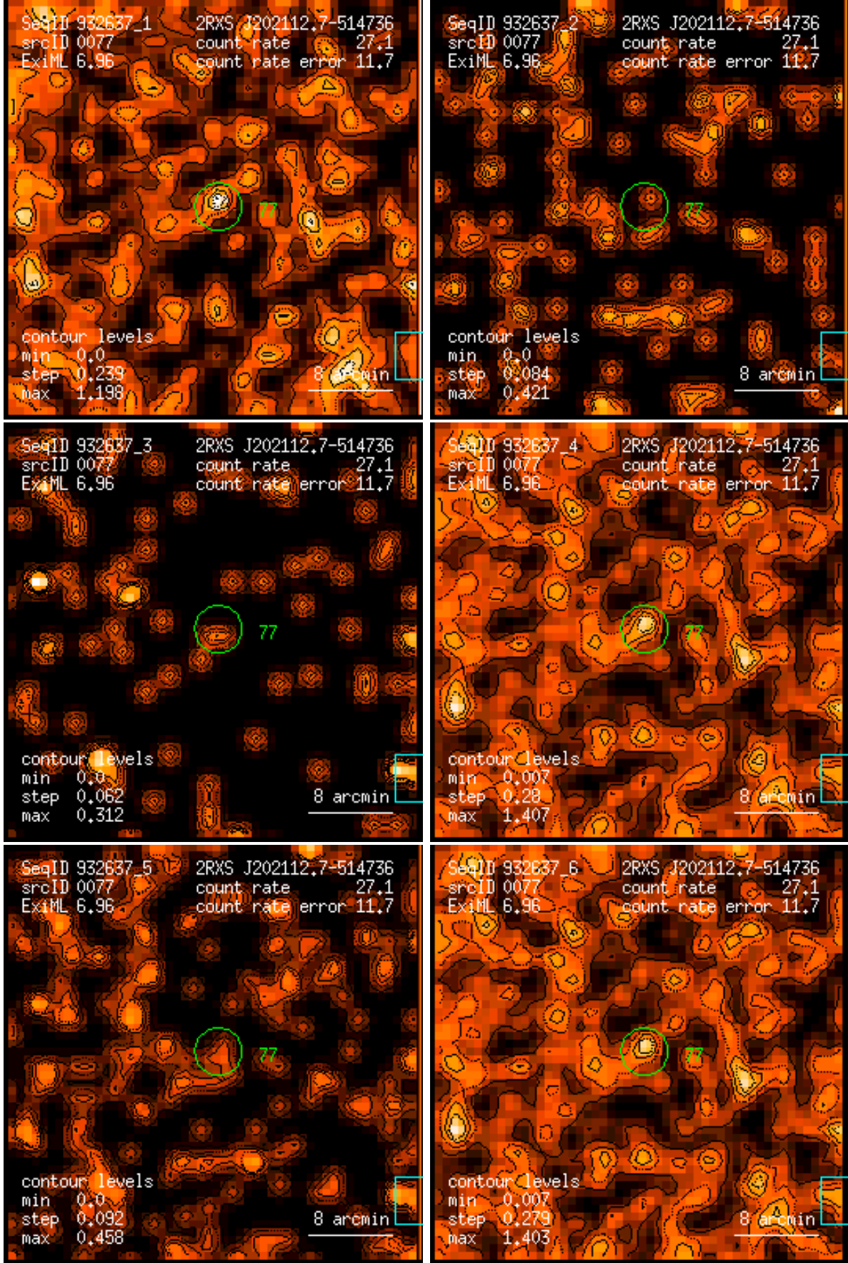
Figure 77: RASS 932637: detection 0077: band rate images, Gaussian filter: (1) PSPC channels 11 – 41, (2) 52 – 90, (3) 91 – 201, (4) 11 – 235, (5) 52 – 201, (6) 11 – 201. Broad band rates in counts/ks. Band rate contour levels in counts/ks/arcmin 2 .
