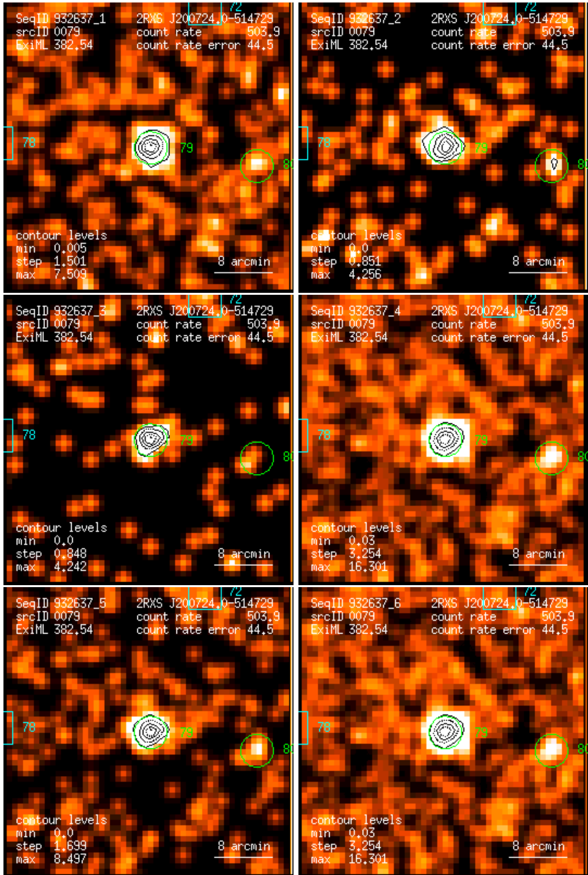
Figure 79: RASS 932637: detection 0079: band rate images, Gaussian filter: (1) PSPC channels 11 – 41, (2) 52 – 90, (3) 91 – 201, (4) 11 – 235, (5) 52 – 201, (6) 11 – 201. Broad band rates in counts/ks. Band rate contour levels in counts/ks/arcmin 2 .
