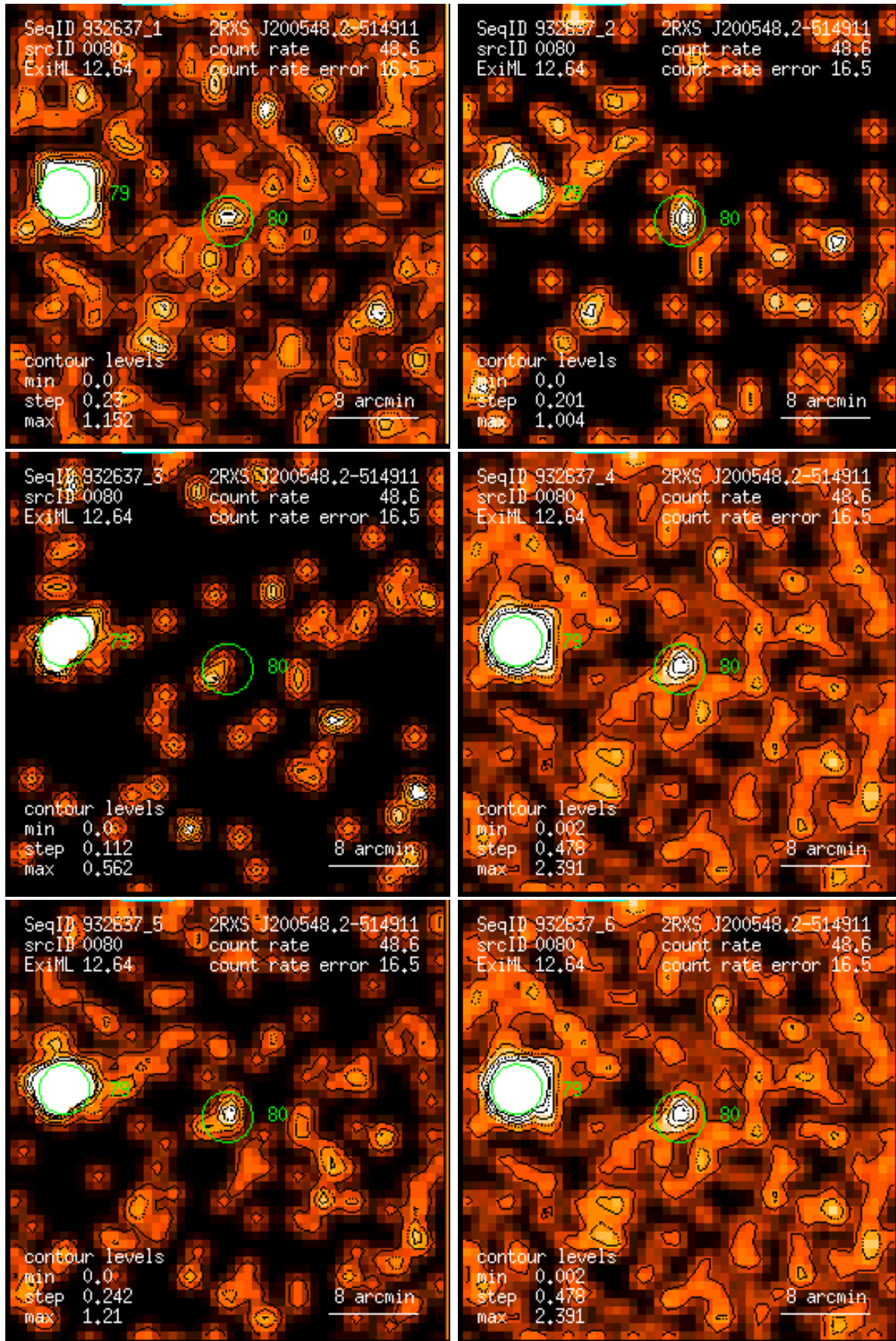
Figure 80: RASS 932637: detection 0080: band rate images, Gaussian filter: (1) PSPC channels 11 – 41, (2) 52 – 90, (3) 91 – 201, (4) 11 – 235, (5) 52 – 201, (6) 11 – 201. Broad band rates in counts/ks. Band rate contour levels in counts/ks/arcmin 2 .
