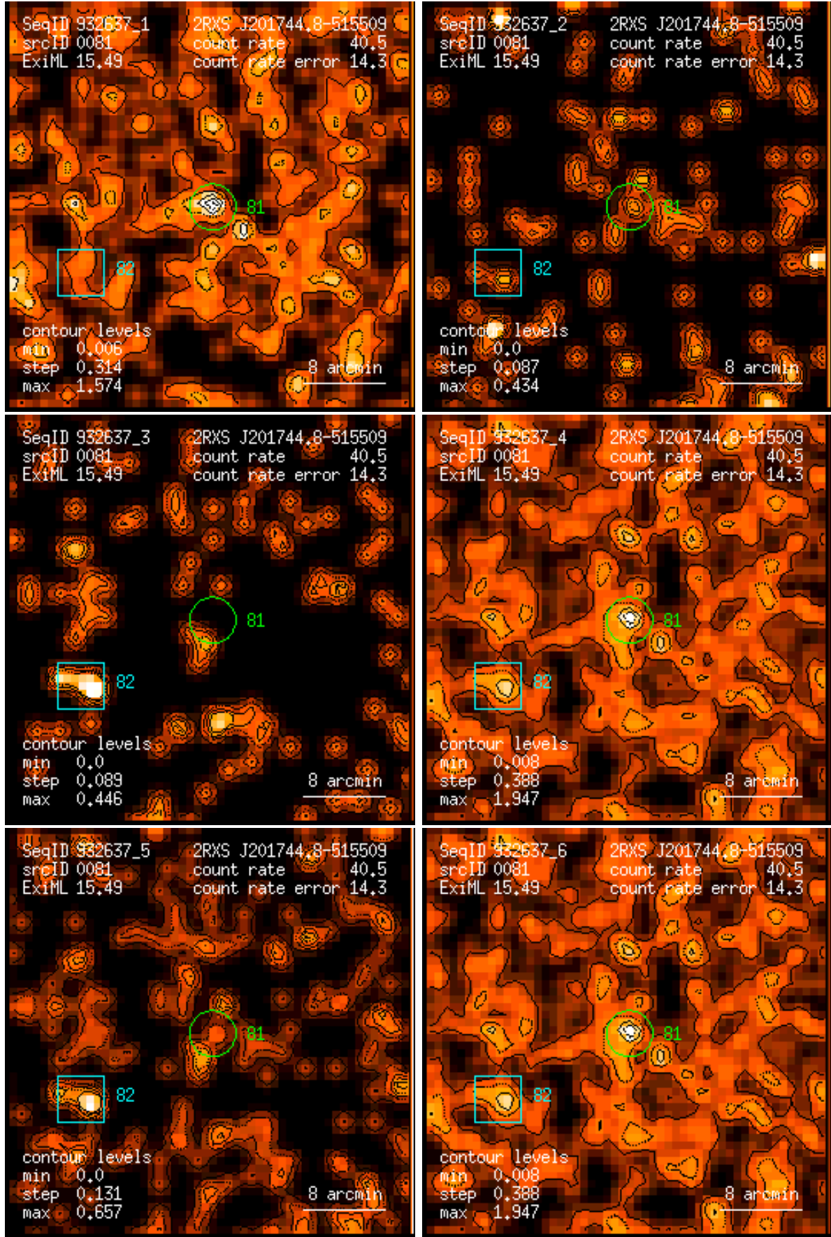
Figure 81: RASS 932637: detection 0081: band rate images, Gaussian filter: (1) PSPC channels 11 – 41, (2) 52 – 90, (3) 91 – 201, (4) 11 – 235, (5) 52 – 201, (6) 11 – 201. Broad band rates in counts/ks. Band rate contour levels in counts/ks/arcmin 2 .
