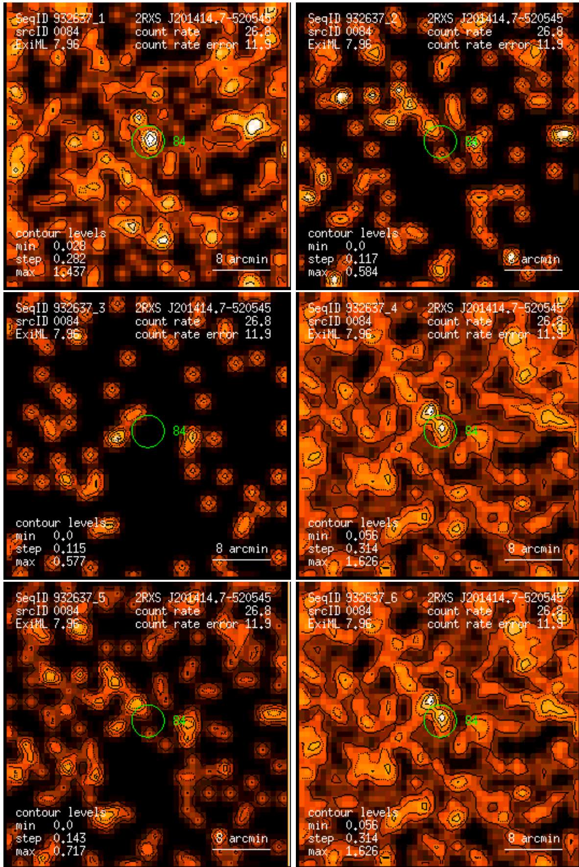
Figure 84: RASS 932637: detection 0084: band rate images, Gaussian filter: (1) PSPC channels 11 – 41, (2) 52 – 90, (3) 91 – 201, (4) 11 – 235, (5) 52 – 201, (6) 11 – 201. Broad band rates in counts/ks. Band rate contour levels in counts/ks/arcmin 2 .
