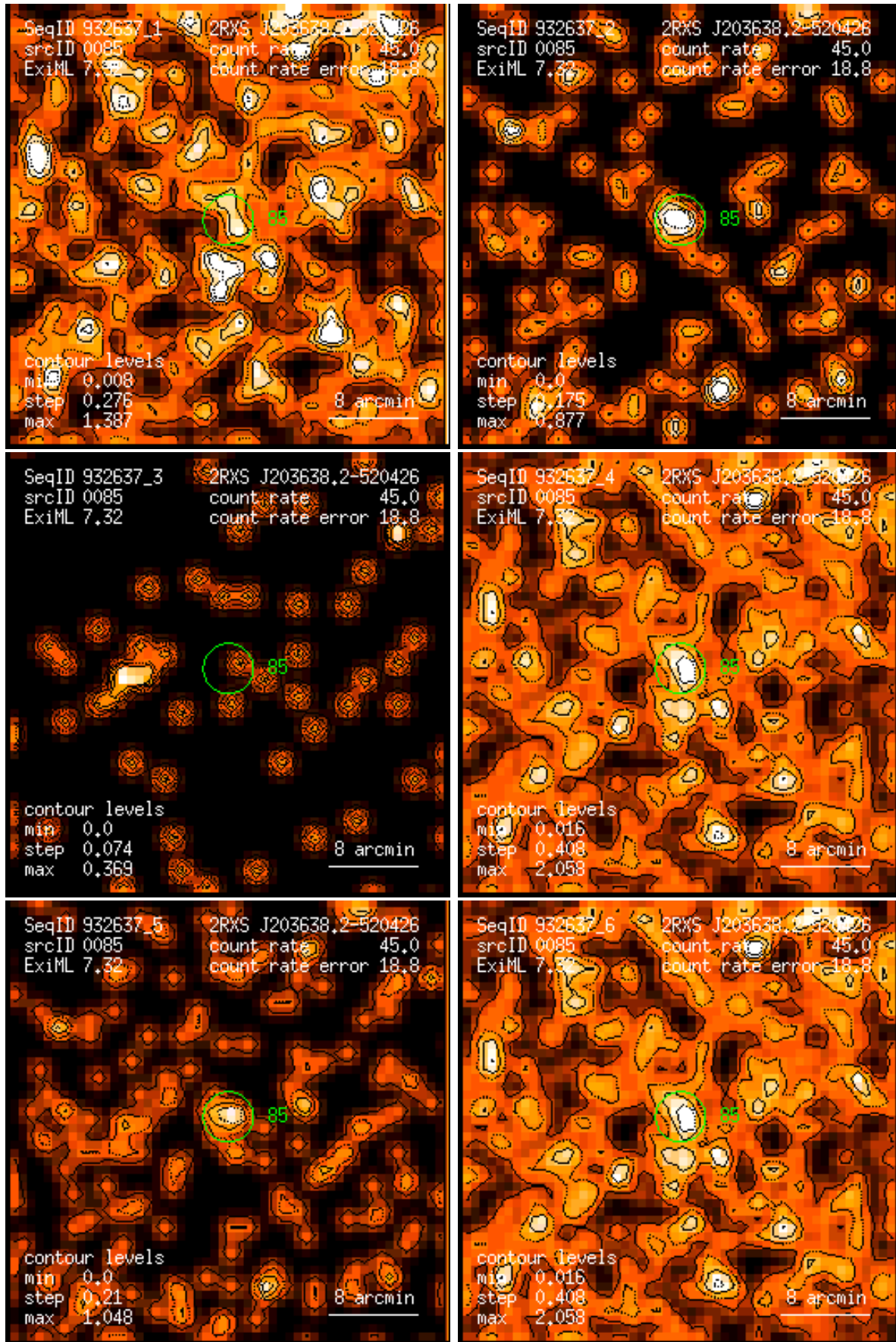
Figure 85: RASS 932637: detection 0085: band rate images, Gaussian filter: (1) PSPC channels 11 – 41, (2) 52 – 90, (3) 91 – 201, (4) 11 – 235, (5) 52 – 201, (6) 11 – 201. Broad band rates in counts/ks. Band rate contour levels in counts/ks/arcmin 2 .
