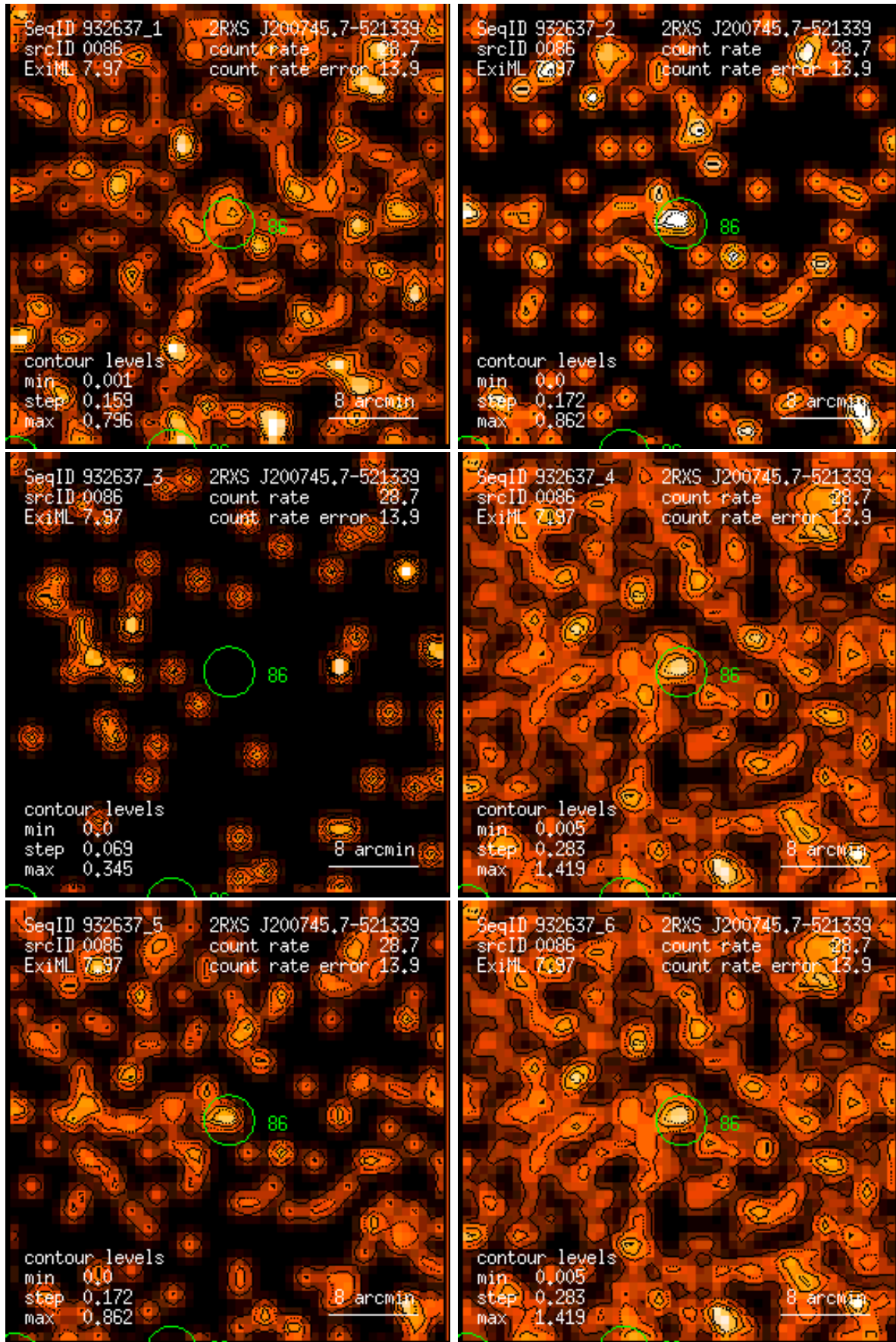
Figure 86: RASS 932637: detection 0086: band rate images, Gaussian filter: (1) PSPC channels 11 – 41, (2) 52 – 90, (3) 91 – 201, (4) 11 – 235, (5) 52 – 201, (6) 11 – 201. Broad band rates in counts/ks. Band rate contour levels in counts/ks/arcmin 2 .
