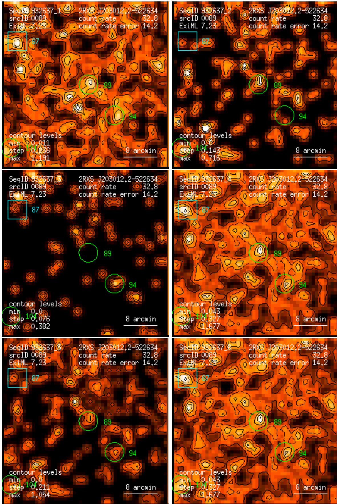
Figure 89: RASS 932637: detection 0089: band rate images, Gaussian filter: (1) PSPC channels 11 – 41, (2) 52 – 90, (3) 91 – 201, (4) 11 – 235, (5) 52 – 201, (6) 11 – 201. Broad band rates in counts/ks. Band rate contour levels in counts/ks/arcmin 2 .
