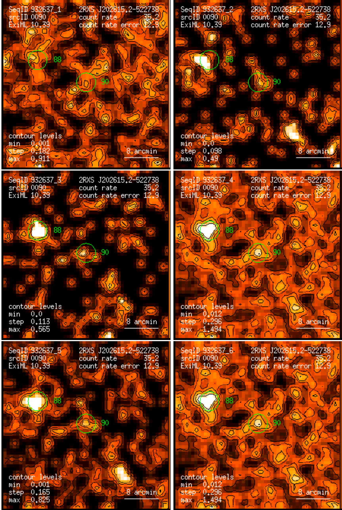
Figure 90: RASS 932637: detection 0090: band rate images, Gaussian filter: (1) PSPC channels 11 – 41, (2) 52 – 90, (3) 91 – 201, (4) 11 – 235, (5) 52 – 201, (6) 11 – 201. Broad band rates in counts/ks. Band rate contour levels in counts/ks/arcmin 2 .
