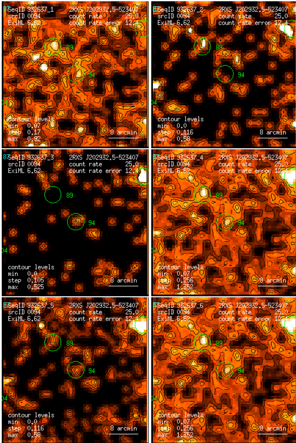
Figure 94: RASS 932637: detection 0094: band rate images, Gaussian filter: (1) PSPC channels 11 – 41, (2) 52 – 90, (3) 91 – 201, (4) 11 – 235, (5) 52 – 201, (6) 11 – 201. Broad band rates in counts/ks. Band rate contour levels in counts/ks/arcmin 2 .
